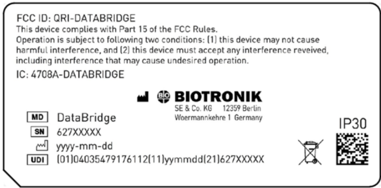
Figure 2: DataBridge type label
