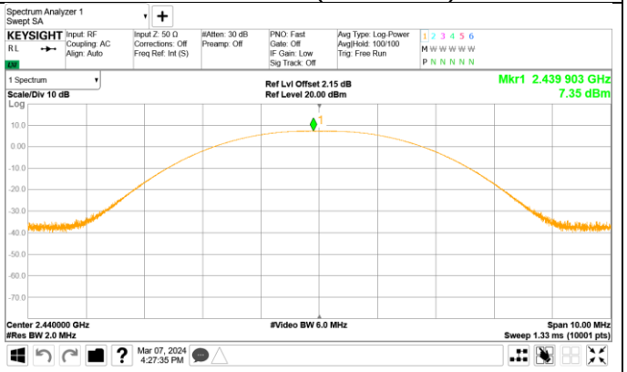
Channel 19 (2440MHz)
