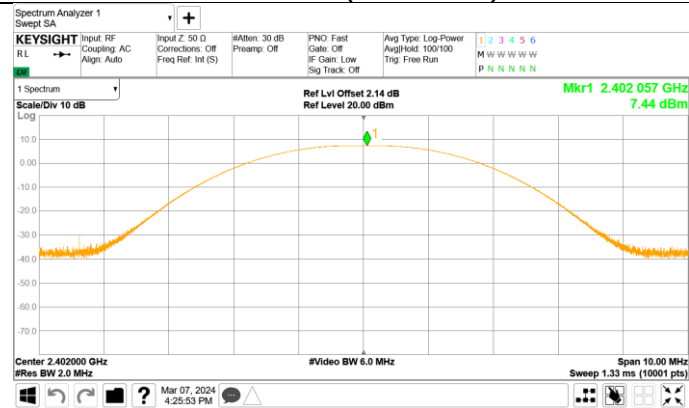
Channel 0 (2402MHz)
