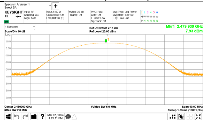
Channel 39 (2480MHz)
