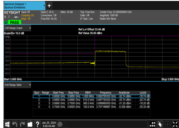
N77(40M)_DFT-s- OFDM_QPSK_Outer_Full_Low_CH
