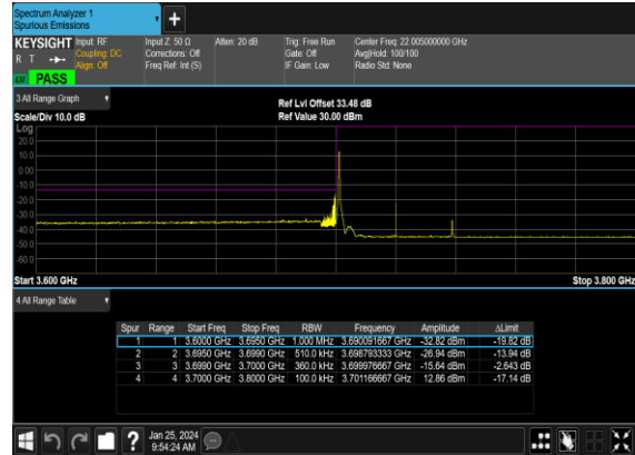
N77(40M)_DFT-s- OFDM_QPSK_Edge_1RB_Left_Low_CH
