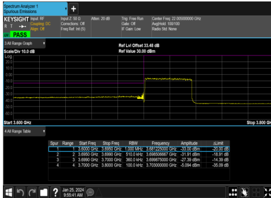
N77(40M)_DFT-s- OFDM_BPSK_Outer_Full_Low_CH
