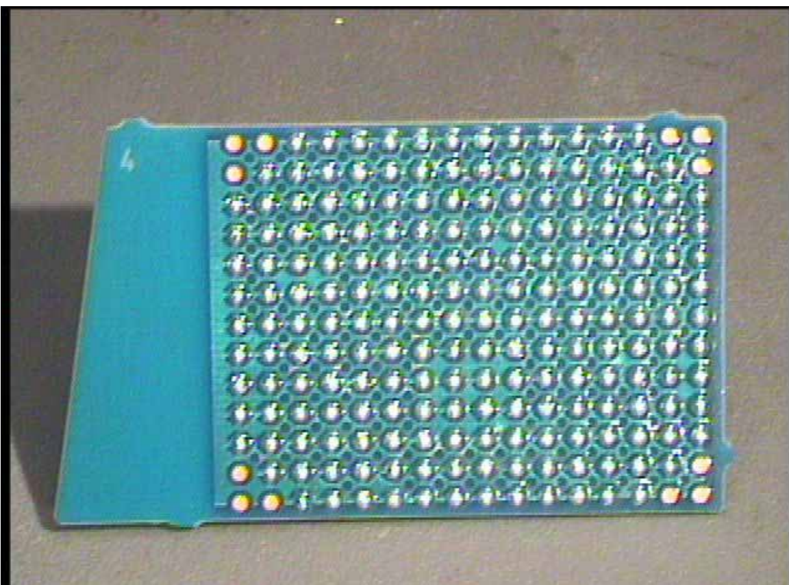
Photo 13 WLAN Module Block - b
