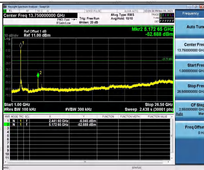
11N40SISO_Ant2_2437_0~Reference
