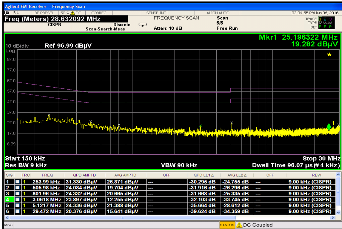
Plot 7-20. Line Conducted Plot with Bluetooth LE (L1)
