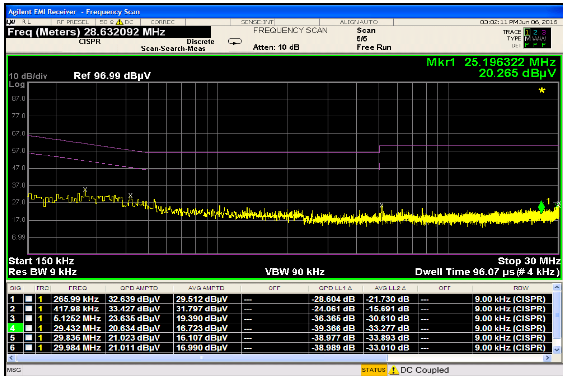
Plot 7-21. Line Conducted Plot with Bluetooth LE (N)
