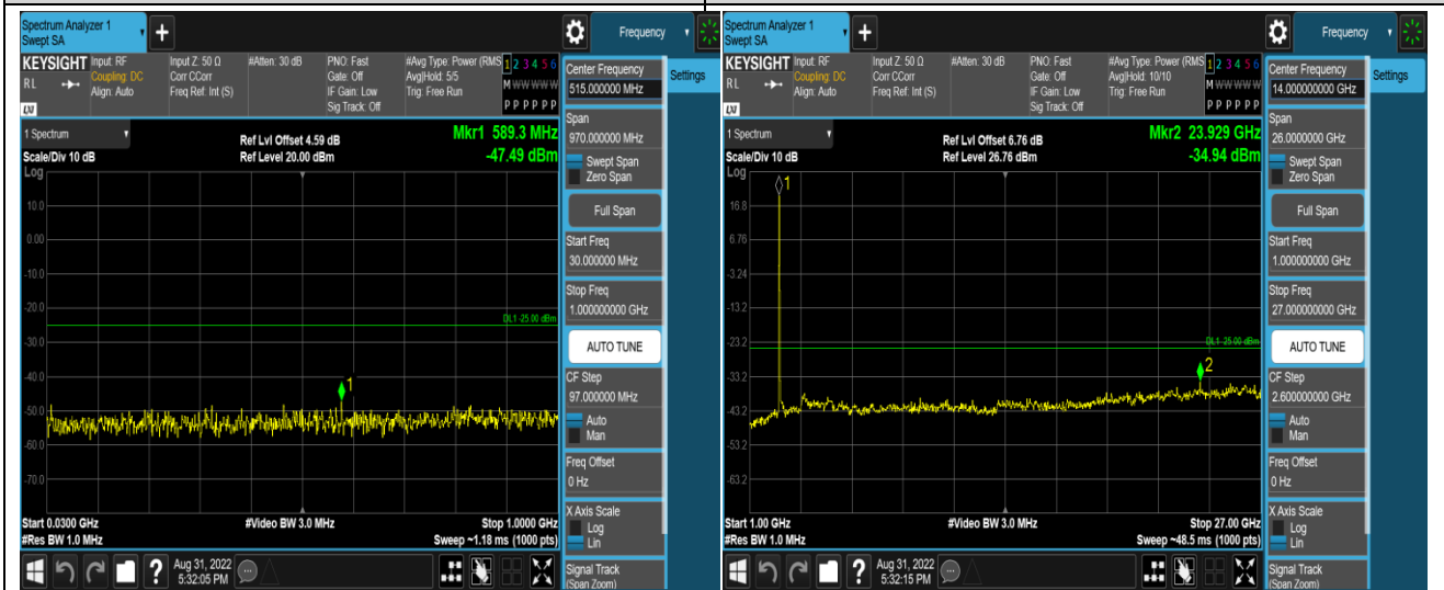
Band41-20MHz-64QAM-39750-100RB#0-Range1:3 30~1000MHz
