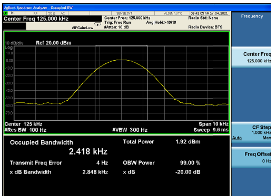
Mobile Phone Charging Antenna 2 Mode
