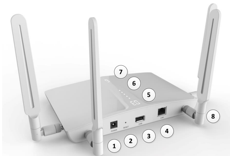
Figure 2-2 second generation ESL Access Point physical interface diagram
