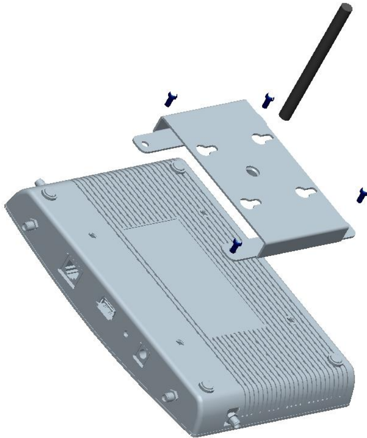
Figure 3-3 ESL Access Point mounting accessories
