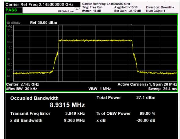
Channel: MIDDLE, Modulation: 256QAM, BW=10MHz
