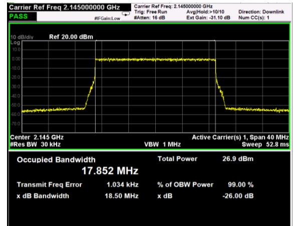
Channel: MIDDLE, Modulation: 256QAM, BW=20MHz
