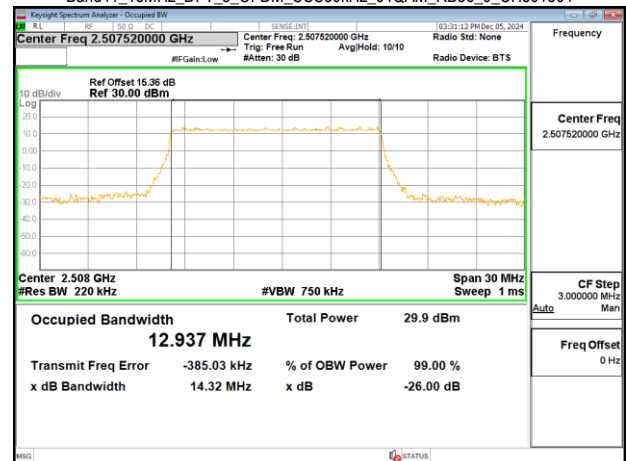
Band41_15MHz_DFT_s_OFDM_SCS30kHz_64QAM_RB36_0_CH501504
