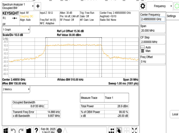
Band53_10MHz_DFT_s_OFDM_SCS30kHz_16QAM_RB24_0_CH497700
