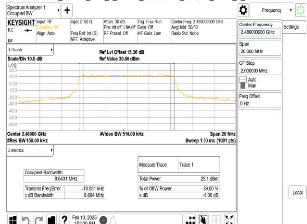
Band53_10MHz_DFT_s_OFDM_SCS30kHz_16QAM_RB24_0_CH497800
