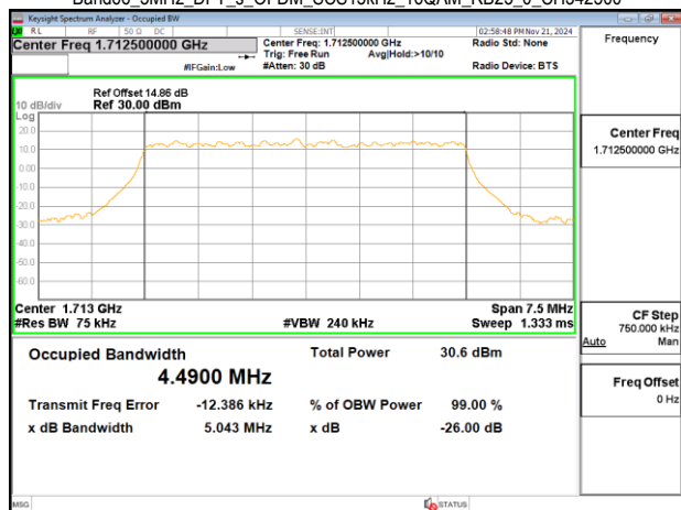
Band66_5MHz_DFT_s_OFDM_SCS15kHz_16QAM_RB25_0_CH342500
