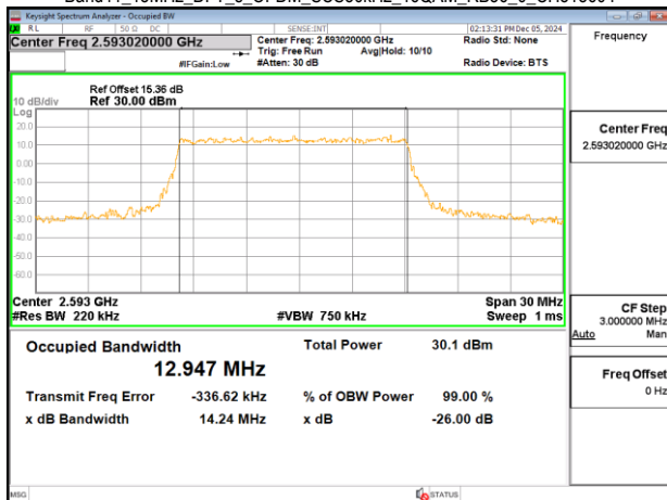
Band41_15MHz_DFT_s_OFDM_SCS30kHz_16QAM_RB36_0_CH518604
