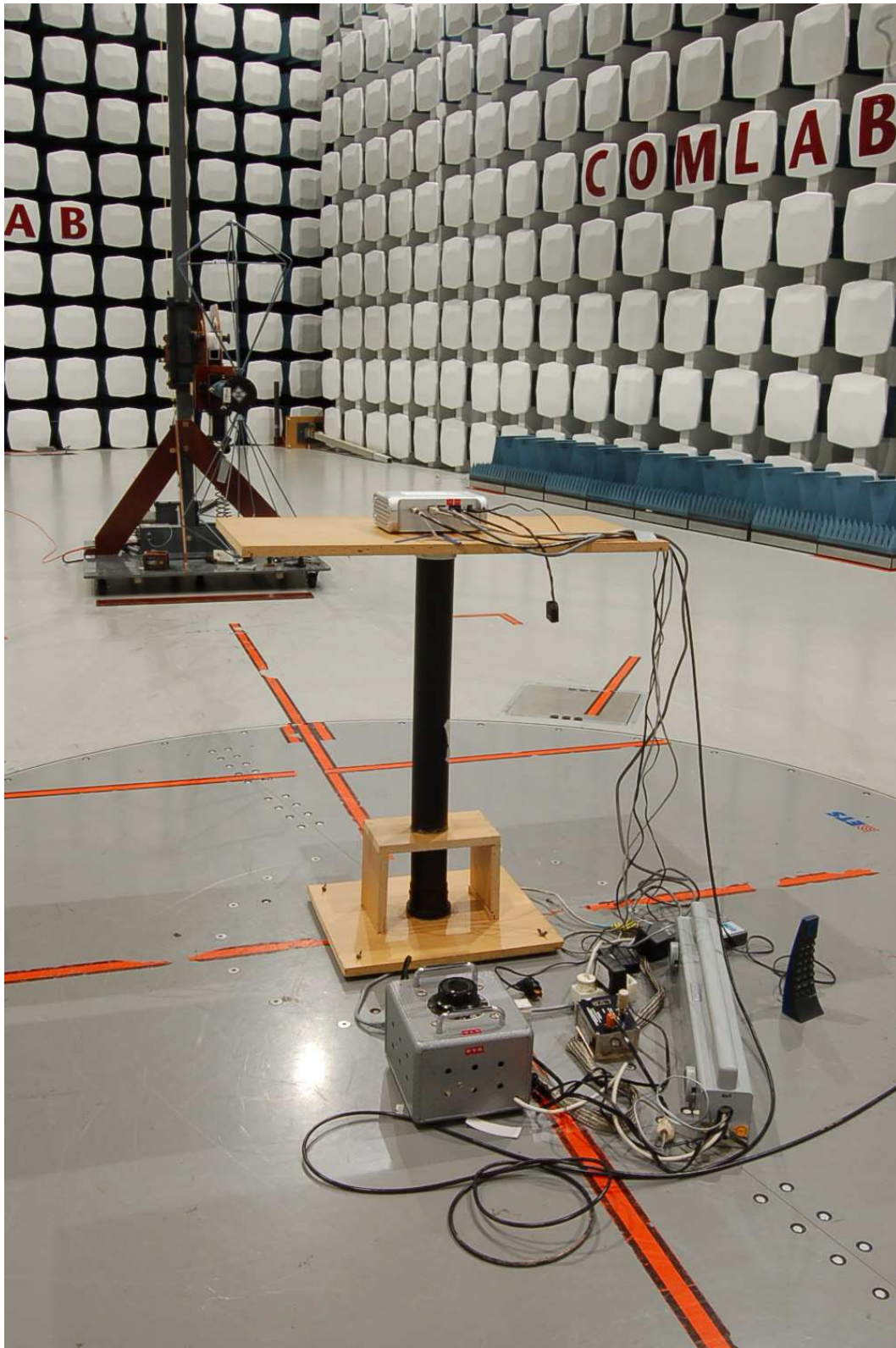
DPC2223 - Radiated emissions test, 3m
