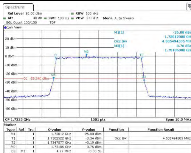
Band4-5MHz-16QAM-20375-25RB#0
