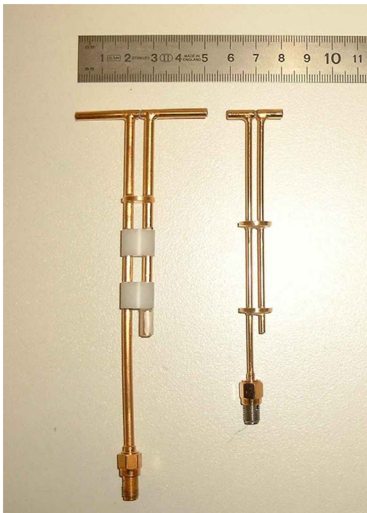
Photo 1: validation dipoles
