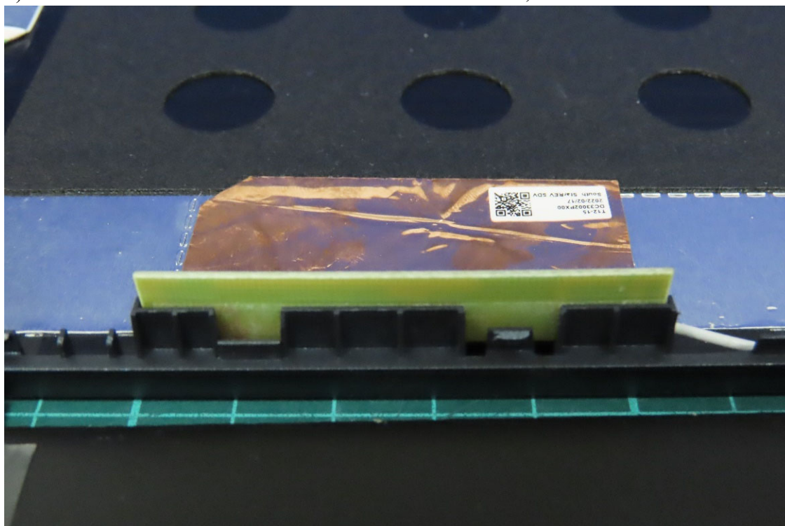
(28) EUT Photo - Antenna: SOUTHSTAR TECHNOLOGY CO.,LTD
