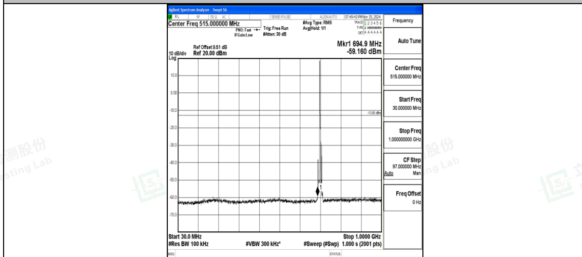
Band12_5MHz_QPSK_23095_1RB#0_30~1000_30~1000
