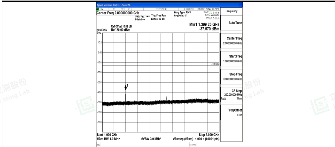
Band12_10MHz_QPSK_23060_1RB#0_1000~3000_1000~3000
