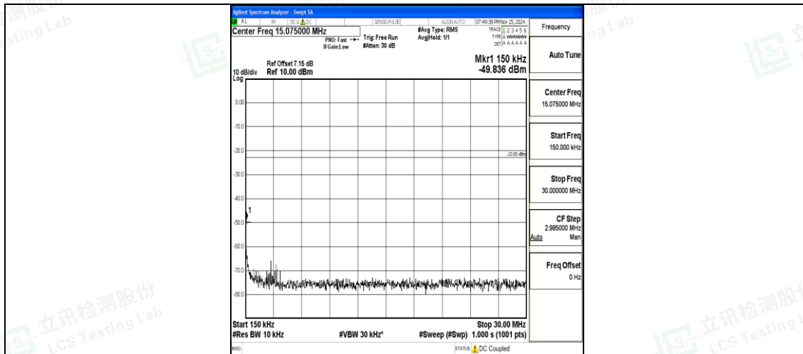
Band12_5MHz_QPSK_23095_1RB#0_0.15~30_0.15~30
