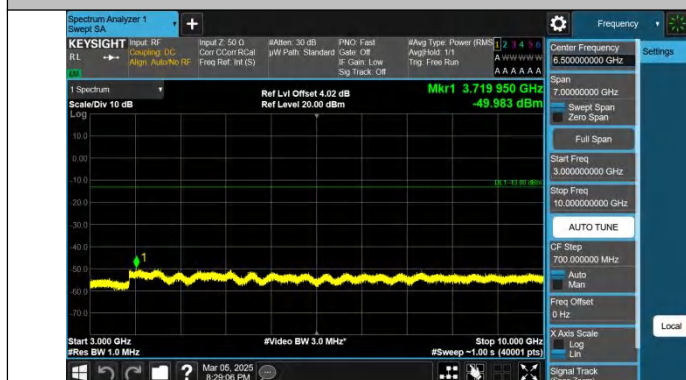
Band5-10MHz-QPSK-20450-1RB#0-3000~10000-PASS
