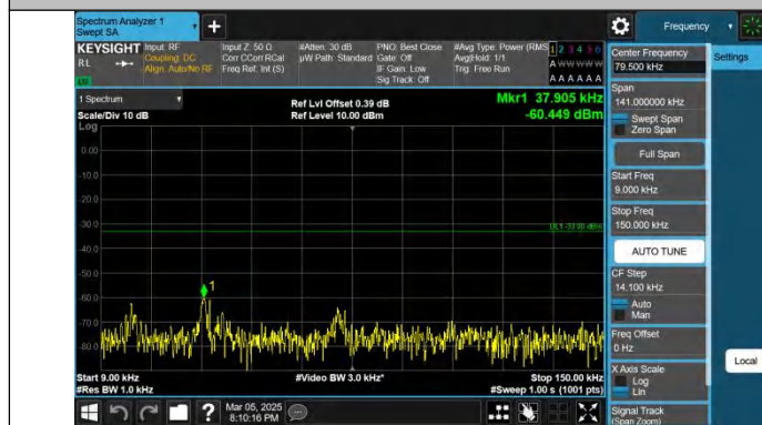
Band5-1.4MHz-QPSK-20643-1RB#0-0.009~0.15-PASS
