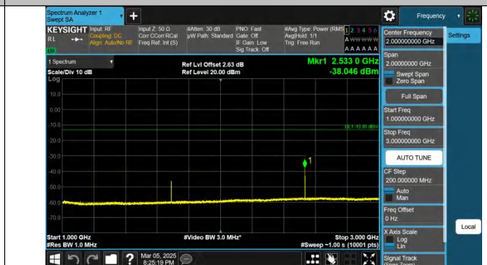
Band5-5MHz-QPSK-20625-1RB#0-1000~3000-PASS
