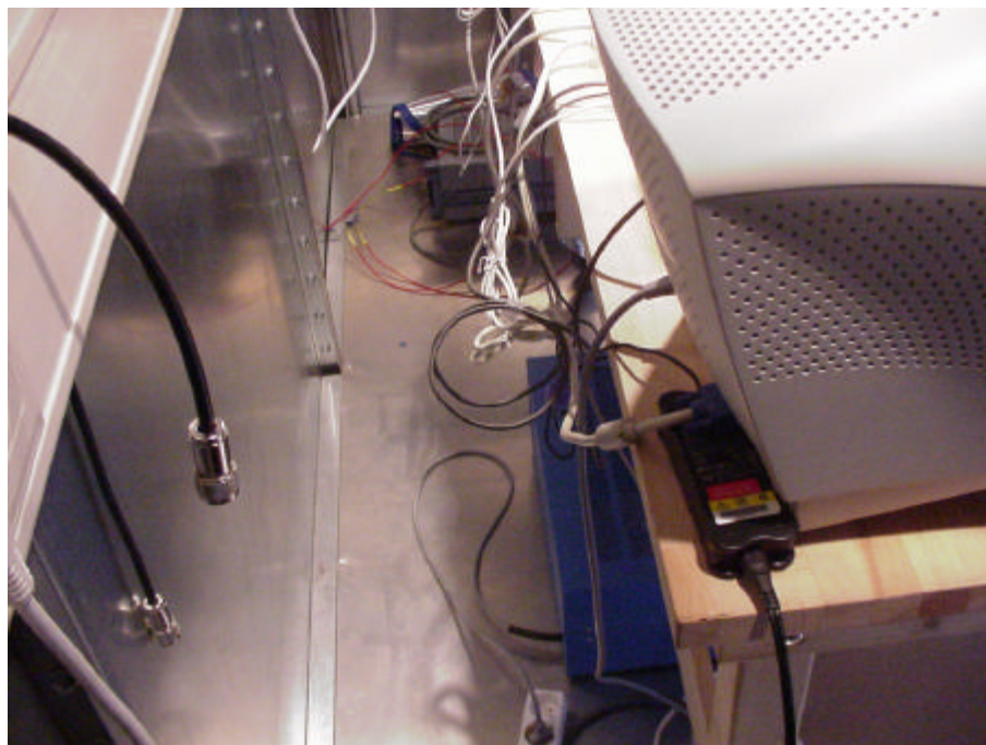
Picture 4 : Setup for emission measurement on the AC mains (rear side)
