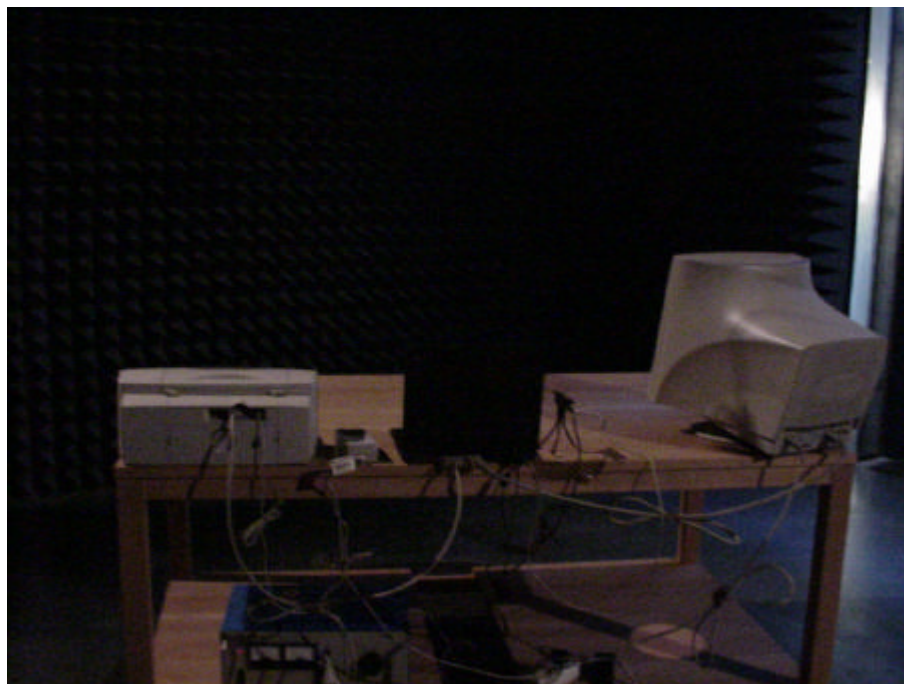
Picture 2 : Setup for radiated emission measurement (rear side)
