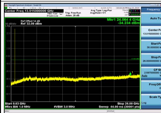
FDD26_LowRange_3MHz_30MHz~26GHz
