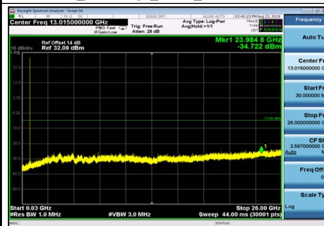
FDD26_MidRange_1.4MHz_30MHz~26GHz
