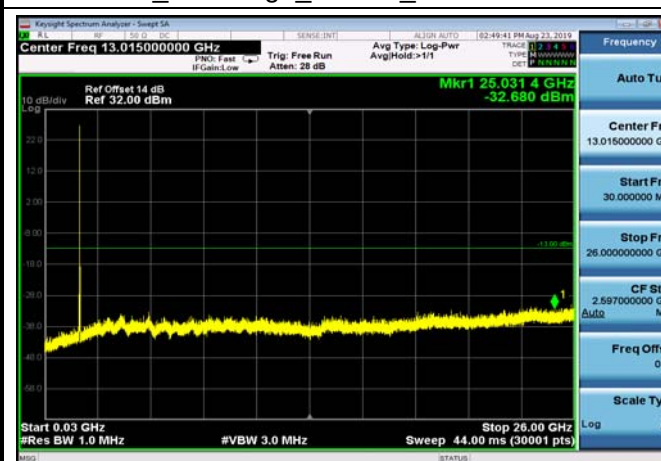
FDD66_MidRange_15MHz_30MHz~26GHz
