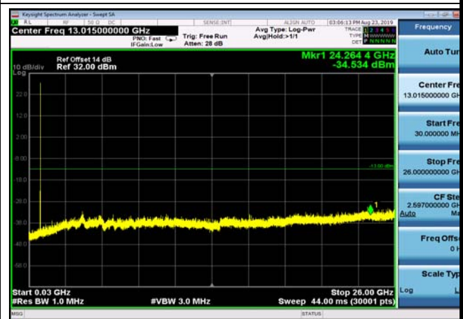
FDD26_HighRange_3MHz_30MHz~26GHz
