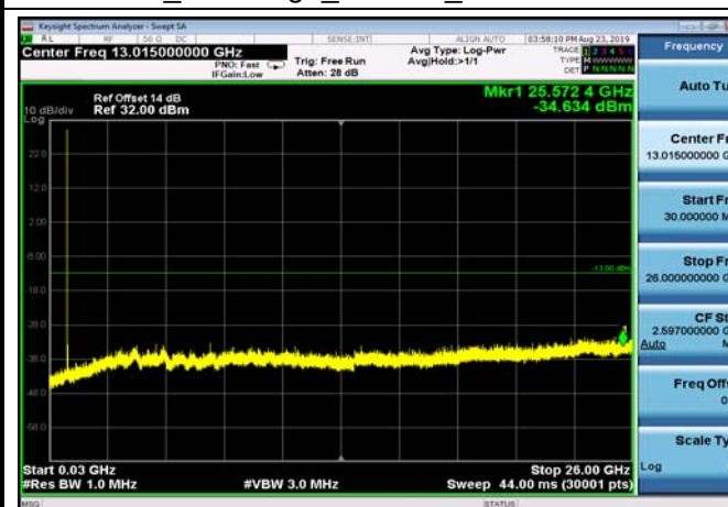
FDD26_MidRange_1.4MHz_30MHz~26GHz
