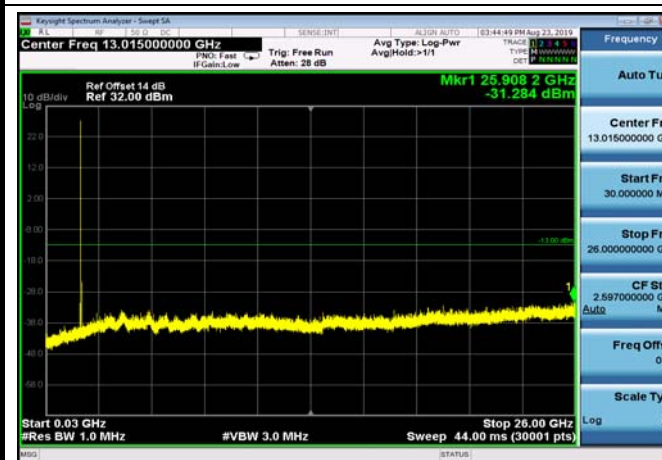
FDD66_LowRange_1.4MHz_30MHz~26GHz
