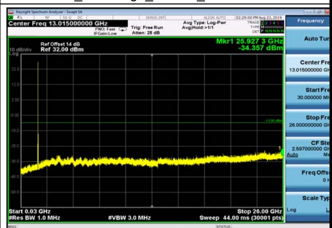
FDD66_MidRange_20MHz_30MHz~26GHz
