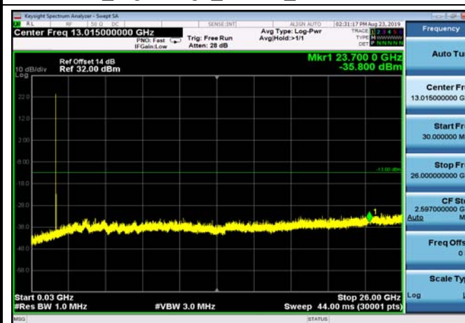
FDD66_HighRange_5MHz_30MHz~26GHz
