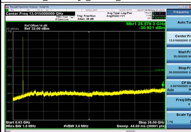
FDD66_LowRange_15MHz_30MHz~26GHz
