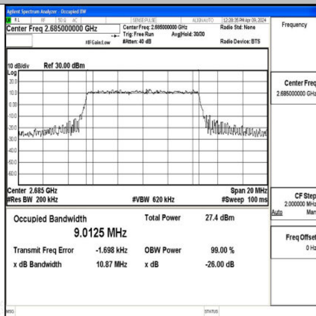
Band41-10MHz-16QAM-41540-50RB#0-PASS
