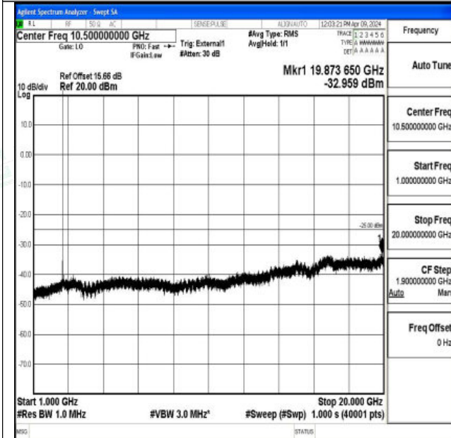
Band41_5MHz_16QAM_40620_1RB#0_1000~20000_100 0~20000
