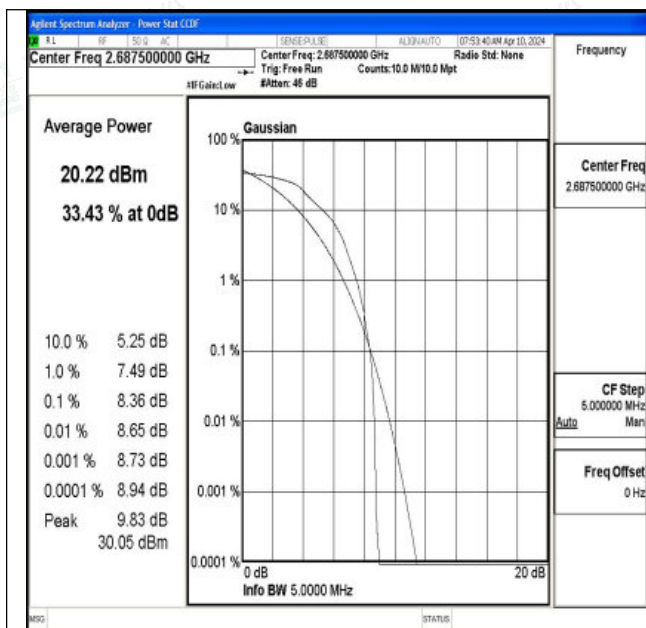
Band41-5MHz-QPSK-41565-1RB#0-PASS
