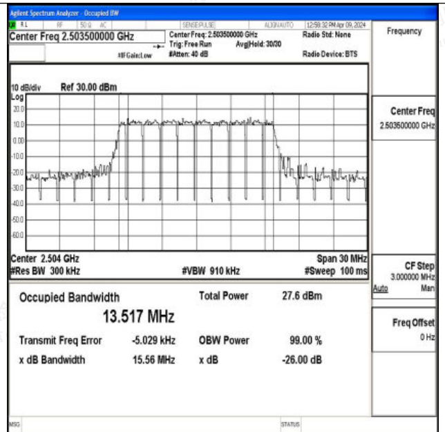
Band41-15MHz-16QAM-39725-75RB#0-PASS
