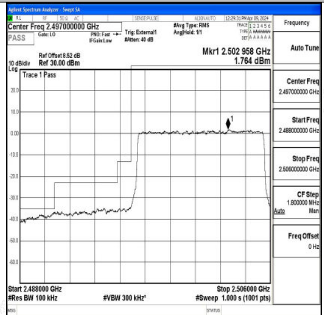
Band41_10MHz_16QAM_39700_50RB#0
