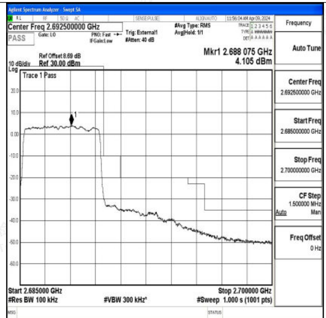
Band41_5MHz_16QAM_41565_25RB#0
