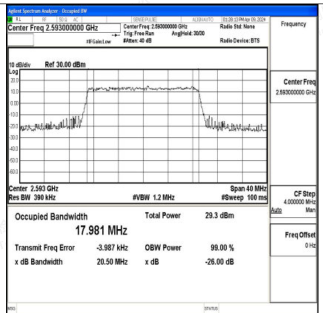
Band41-20MHz-16QAM-40620-100RB#0-PASS
