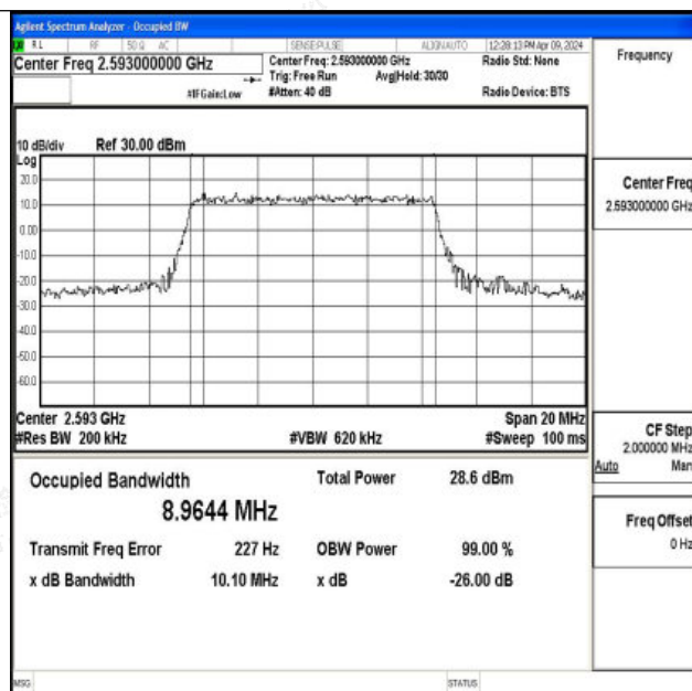
Band41-10MHz-16QAM-40620-50RB#0-PASS
