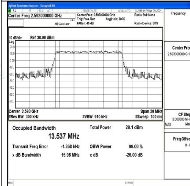
Band41-15MHz-QPSK-40620-75RB#0-PASS
