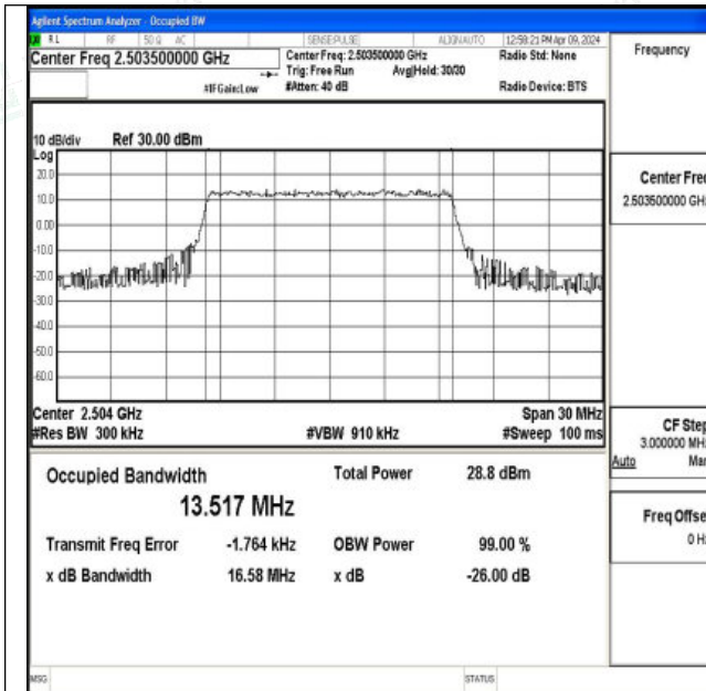
Band41-15MHz-QPSK-39725-75RB#0-PASS
