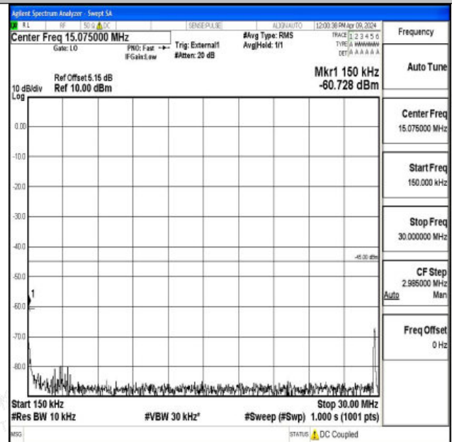
Band41_5MHz_QPSK_40620_1RB#0_0.15~30_0.15~30
