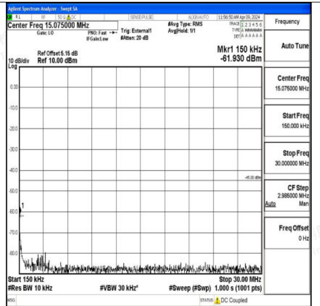
Band41_5MHz_QPSK_39675_1RB#0_0.15~30_0.15~30
