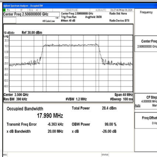
Band41-20MHz-16QAM-39750-100RB#0-PASS
