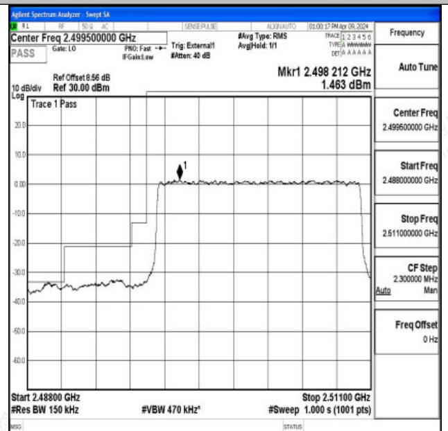
Band41_15MHz_16QAM_39725_75RB#0
