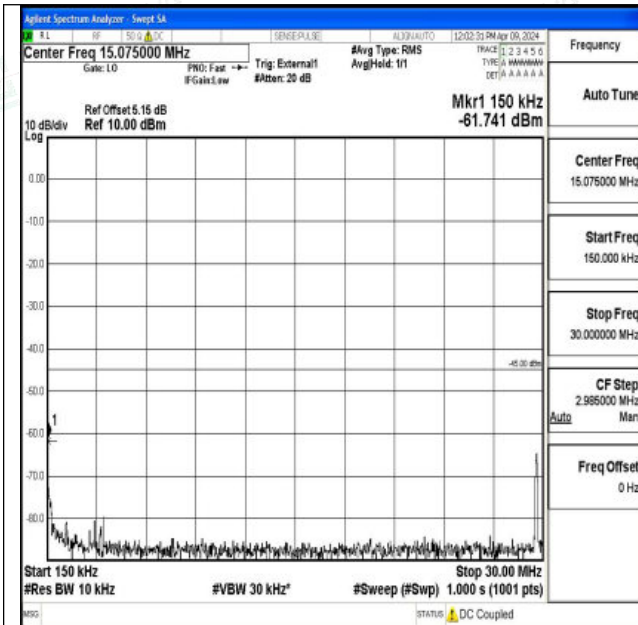
Band41_5MHz_16QAM_40620_1RB#0_0.15~30_0.15~30
