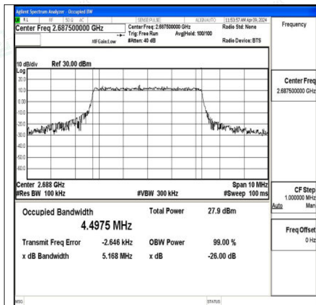
Band41-5MHz-QPSK-41565-25RB#0-PASS
