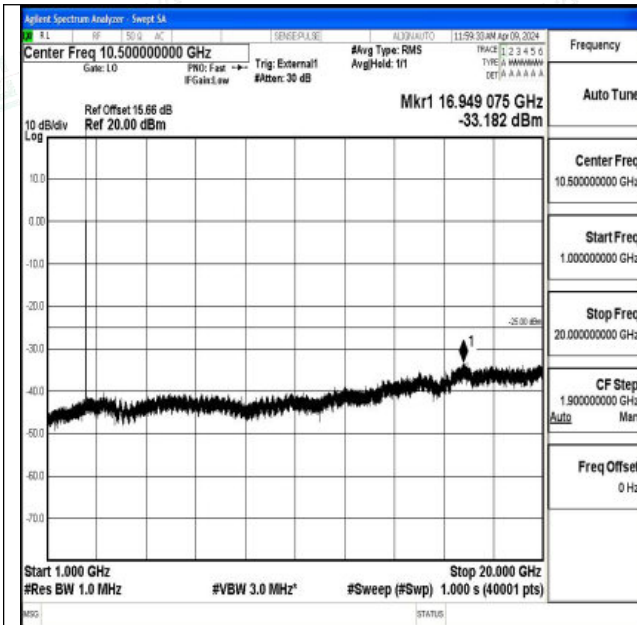
Band41_5MHz_16QAM_39675_1RB#0_1000~20000_100 0~20000
