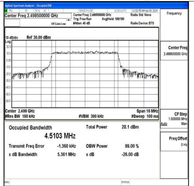
Band41-5MHz-16QAM-39675-25RB#0-PASS
