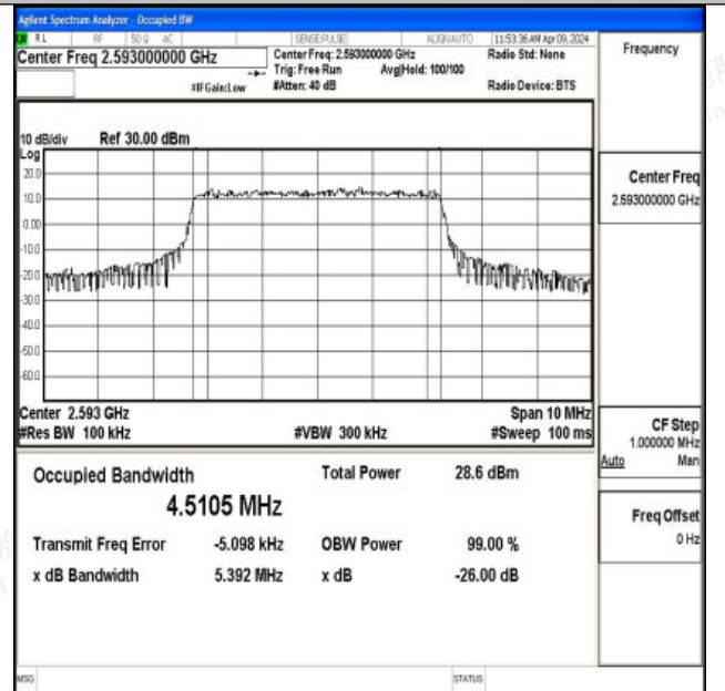
Band41-5MHz-16QAM-40620-25RB#0-PASS
