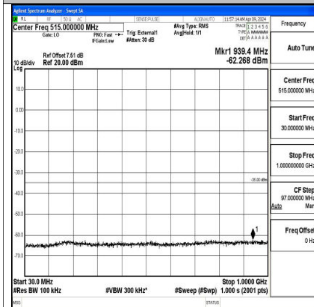
Band41_5MHz_QPSK_39675_1RB#0_30~1000_30~1000
