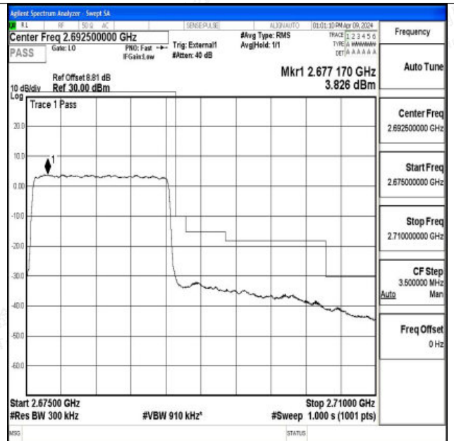
Band41_15MHz_16QAM_41515_75RB#0
