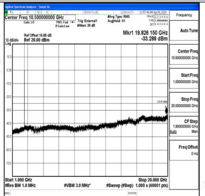
Band41_5MHz_QPSK_39675_1RB#0_1000~20000_1000~
