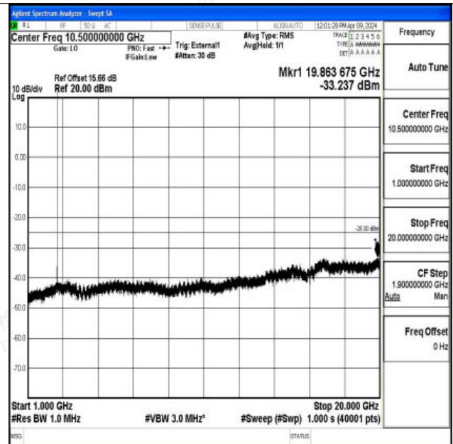
Band41_5MHz_QPSK_40620_1RB#0_1000~20000_1000~20000
