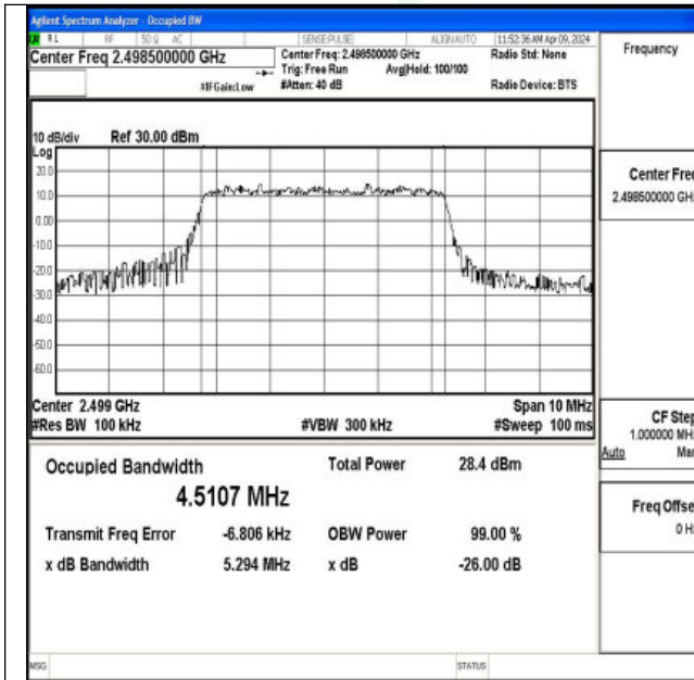
Band41-5MHz-QPSK-39675-25RB#0-PASS
