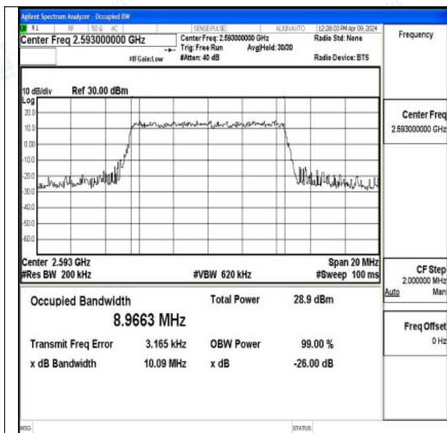
Band41-10MHz-QPSK-40620-50RB#0-PASS
