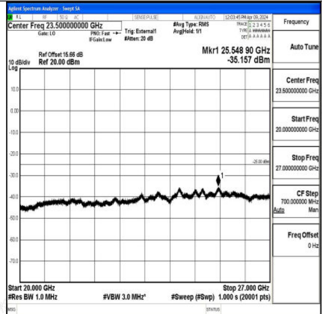
Band41_5MHz_16QAM_40620_1RB#0_20000~27000_200 00~27000
