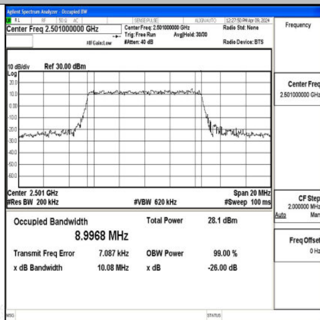
Band41-10MHz-16QAM-39700-50RB#0-PASS
