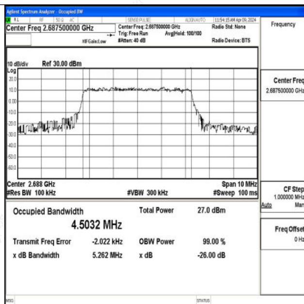
Band41-5MHz-16QAM-41565-25RB#0-PASS
