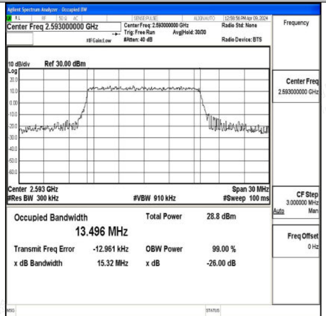
Band41-15MHz-16QAM-40620-75RB#0-PASS
