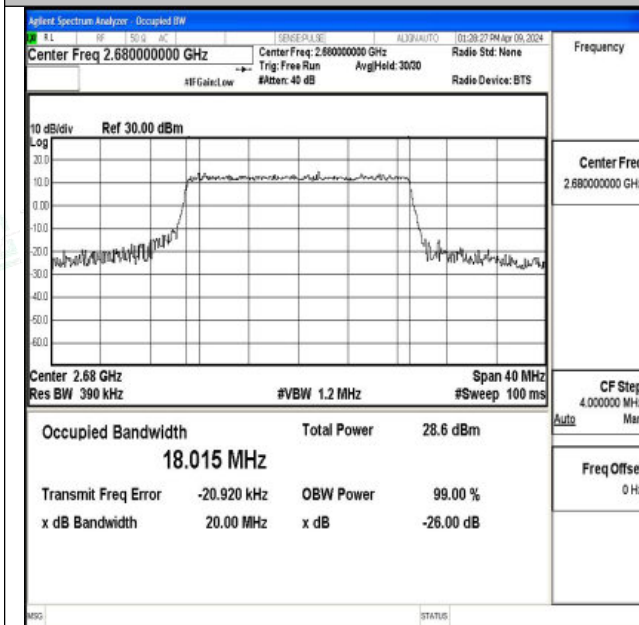
Band41-20MHz-QPSK-41490-100RB#0-PASS
