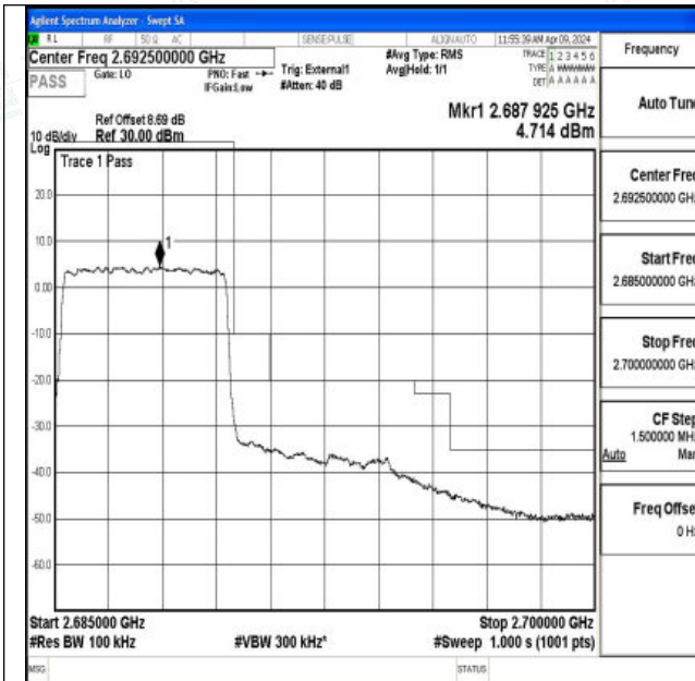
Band41_5MHz_QPSK_41565_25RB#0
