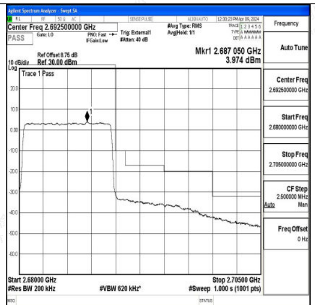
Band41_10MHz_16QAM_41540_50RB#0
