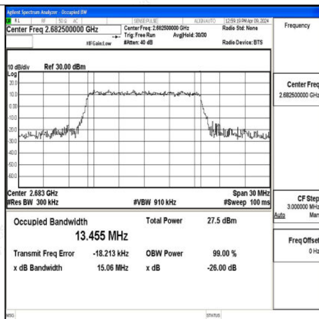
Band41-15MHz-16QAM-41515-75RB#0-PASS
