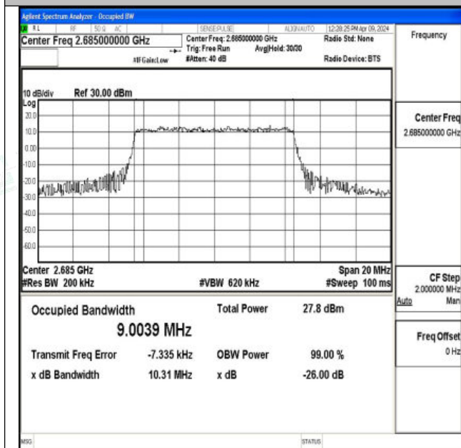
Band41-10MHz-QPSK-41540-50RB#0-PASS
