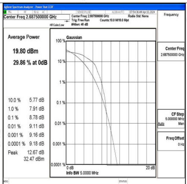
Band41-5MHz-16QAM-41565-1RB#0-PASS
