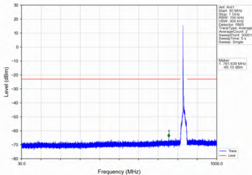
n5_30kHz_SISO_NTNV_10MHz_CP-OFDM_QPSK_836.5MHz_Edge_1RB_Left
