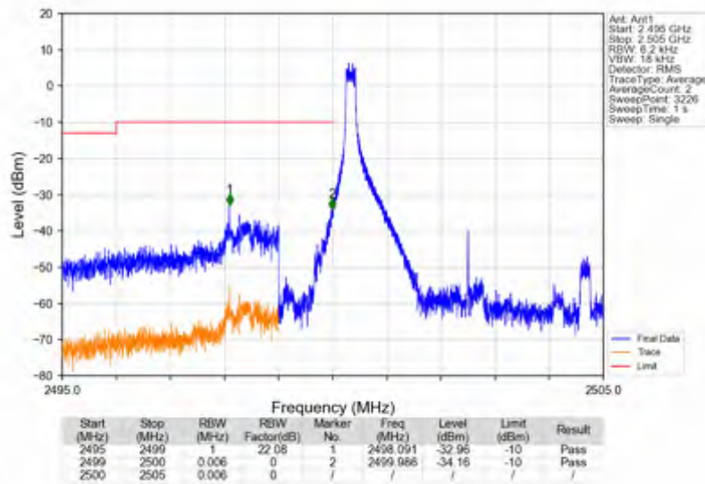
n7_15kHz_SISO_NTNV_5MHz_DFT-s-OFDM_PI/2_BPSK_2502.5MHz_Edge_1RB_Left
