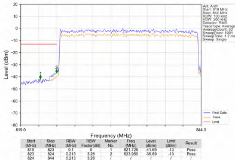
n5_15kHz_SISO_NTNV_20MHz_CP-OFDM QPSK_834MHz_Outer_Full
