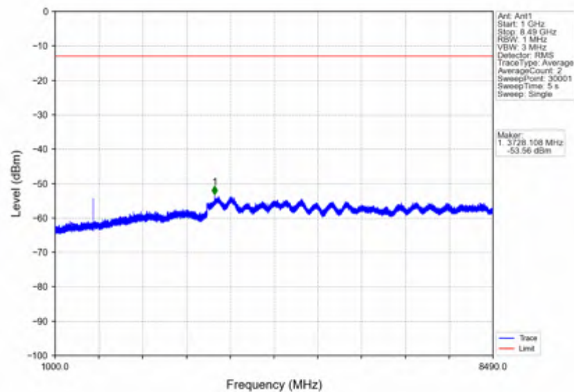
n5_30kHz_SISO_NTNV_10MHz_CP-OFDM QPSK_836.5MHz_Edge_1RB_Left
