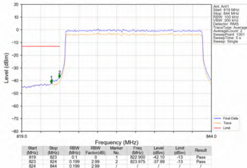
n5_30kHz_SISO_NTNV_20MHz_DFT-s-OFDM QPSK_834MHz_Outer_Full
