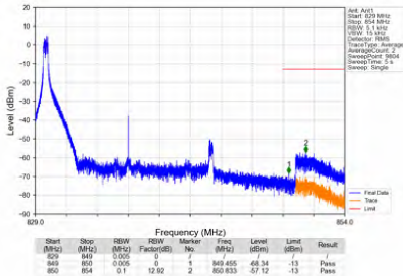
n5_30kHz_SISO_NTNV_15MHz_DFT-s-OFDM_QPSK_836.5MHz_Edge_1RB_Left
