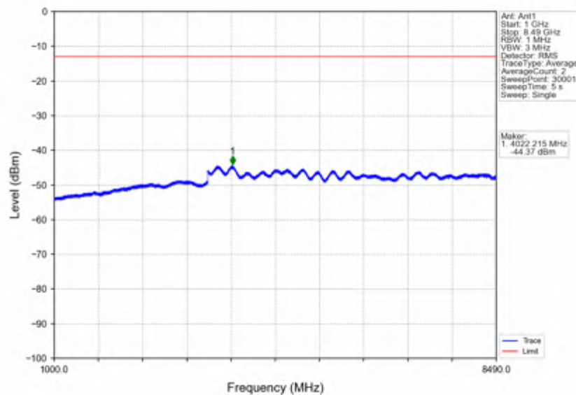
n5 30kHz SISO NTV 20MHz CP-OFDM QPSK 839MHz Outer Full
