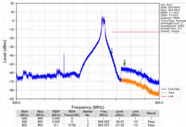
n5_30kHz_SISO_NTNV_10MHz_DFT-s-OFDM PI/2 BPSK_844MHz_Edge_1RB_Right
