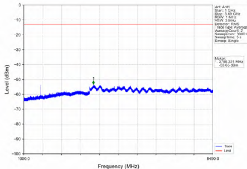
n5_30kHz_SISO_NTNV_10MHz_DFT-s-OFDM PI/2 BPSK_829MHz_Outer_Full
