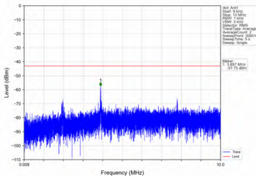
n5_30kHz_SISO_NTNV_20MHz_DFT-s-OFDM QPSK_834MHz_Outer_Full
