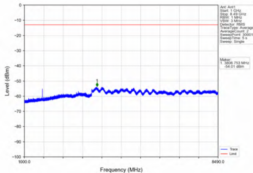
n5_30kHz_SISO_NTV_15MHz_CP-OFDM_QPSK_841.5MHz_Outer_Full
