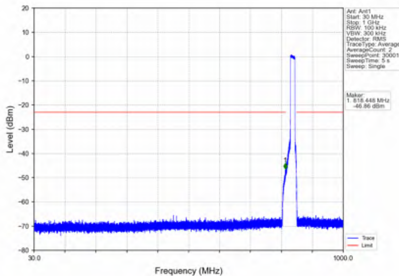
n5_30kHz_SISO_NTNV_15MHz_CP-OFDM_QPSK_841.5MHz_Outer_Full
