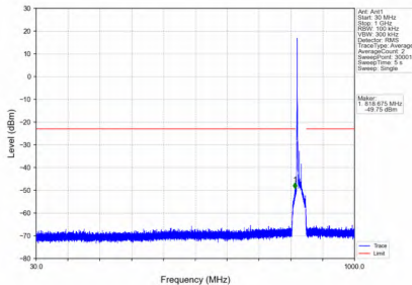
n5_30kHz_SISO_NTV_15MHz_CP-OFDM_QPSK_831.5MHz_Inner_1RB_Left
