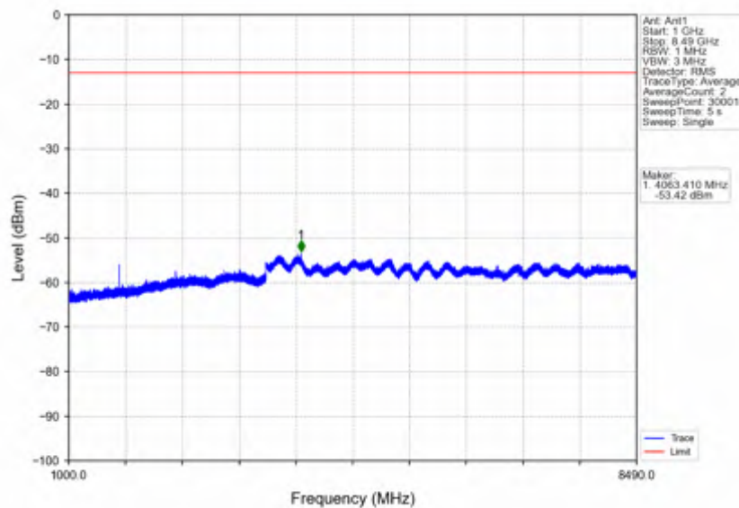
n5_30kHz_SISO_NTNV_10MHz_CP-OFDM_QPSK_836.5MHz_Edge_1RB_Left
