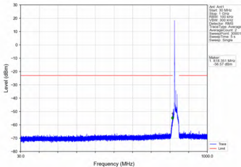
n5_30kHz_SISO_NTNV_15MHz_DFT-s-OFDM_QPSK_836.5MHz_Edge_1RB_Left
