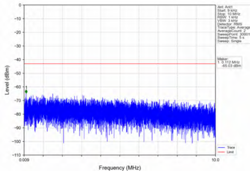
n5_30kHz_SISO_NTNV_15MHz_CP-OFDM_QPSK_841.5MHz_Outer_Full
