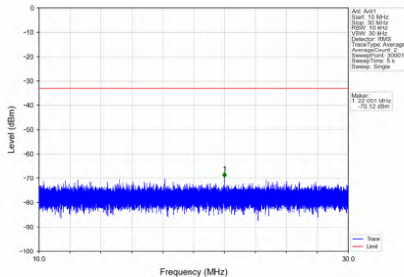
n5_30kHz_SISO_NTNV_15MHz_CP-OFDM QPSK_836.5MHz_Edge_1RB_Left
