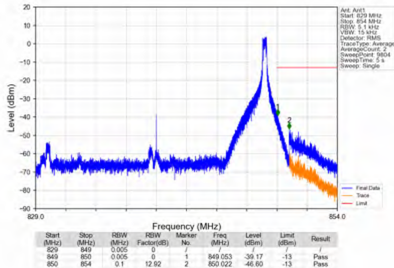
n5_30kHz_SISO_NTNV_20MHz_DFT-s-OFDM_QPSK_839MHz_Edge_1RB_Right
