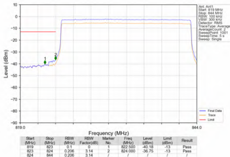
n5_30kHz_SISO_NTNV_20MHz_CP-OFDM QPSK_834MHz_Outer_Full
