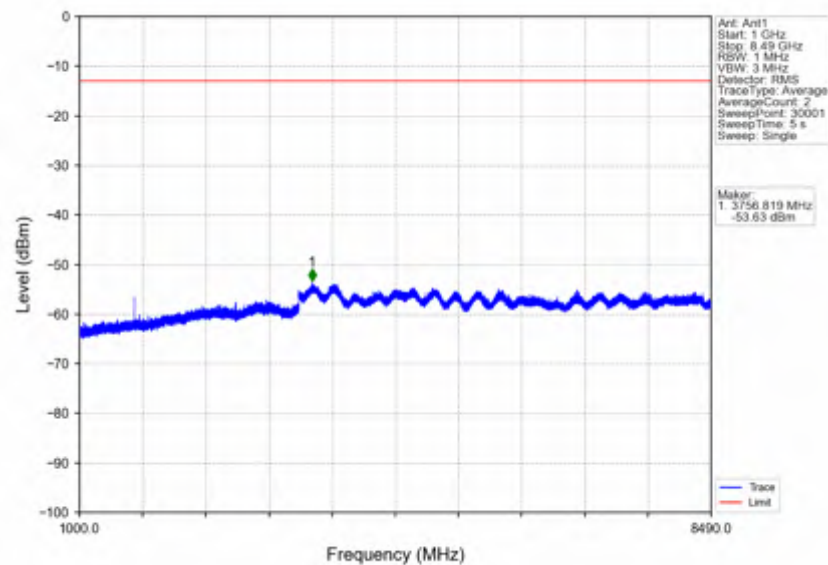
n5_30kHz_SISO_NTNV_20MHz_CP-OFDM QPSK_834MHz_Outer_Full
