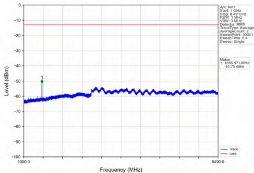
n5_30kHz_SISO_NTNV_15MHz_DFT-s-OFDM QPSK_831.5MHz_Edge_1RB_Left
