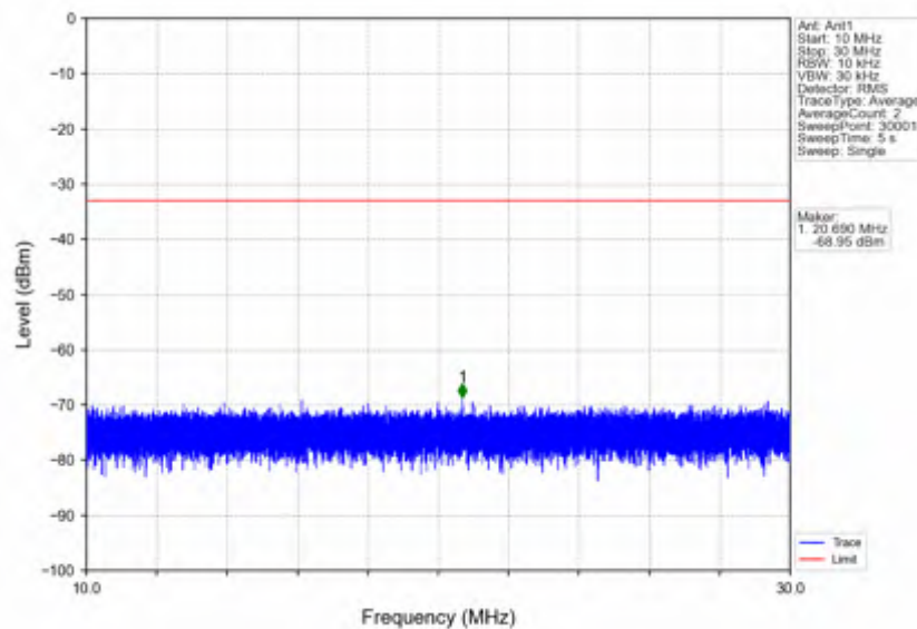
n5_30kHz_SISO_NTNV_20MHz_DFT-s-OFDM QPSK_839MHz_Outer_Full
