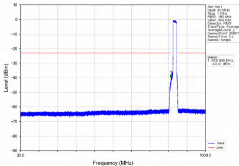
n5 30kHz SISO NTV 20MHz CP-OFDM QPSK 839MHz Outer Full
