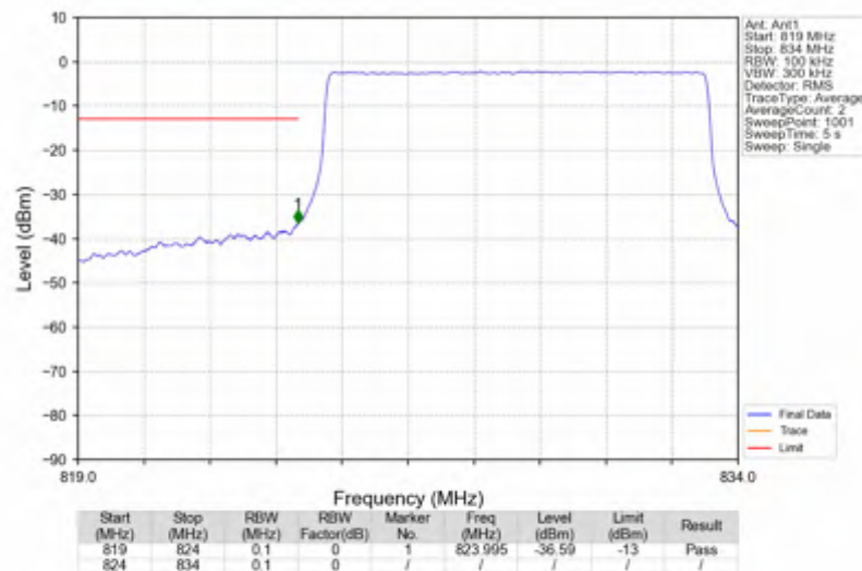
n5_30kHz_SISO_NTNV_10MHz_CP-OFDM QPSK_829MHz_Outer_Full
