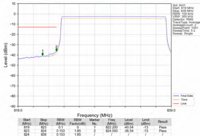
n5_30kHz_SISO_NTNV_15MHz_CP-OFDM QPSK_831.5MHz_Outer_Full
