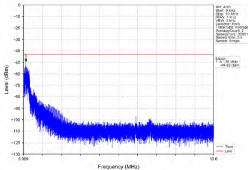
n5_30kHz_SISO_NTNV_15MHz_DFT-s-OFDM_QPSK_836.5MHz_Edge_1RB_Left
