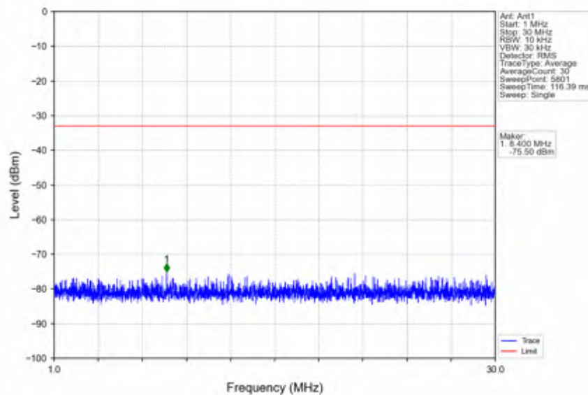
n5_15kHz_SISO_NTNV_20MHz_CP-OFDM QPSK_839MHz_Edge_1RB_Right
