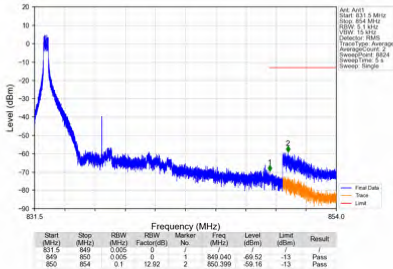
n5_30kHz_SISO_NTNV_10MHz_DFT-s-OFDM_QPSK_836.5MHz_Edge_1RB_Left
