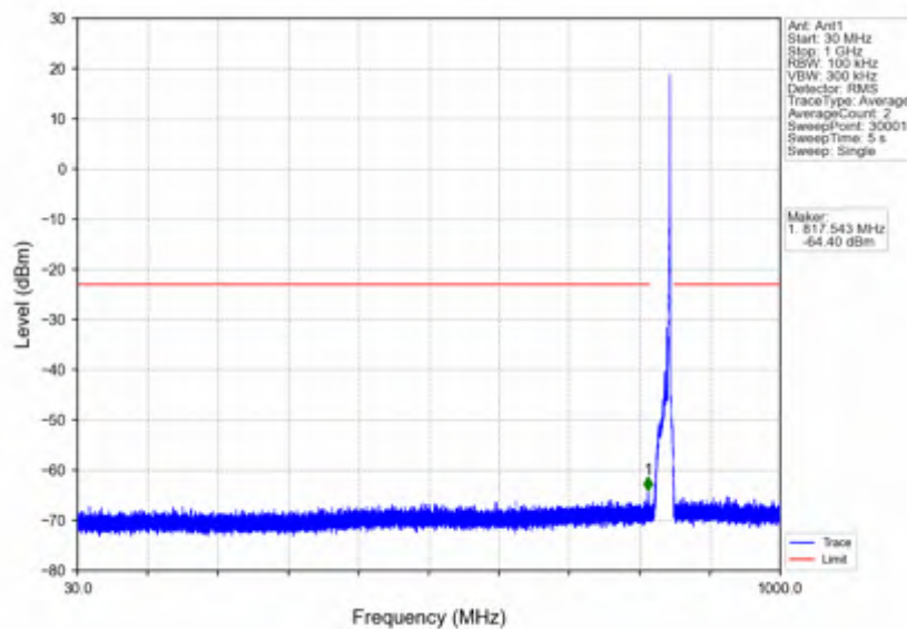
n5_30kHz_SISO_NTNV_10MHz_DFT-s-OFDM_QPSK_844MHz_Inner_1RB_Right
