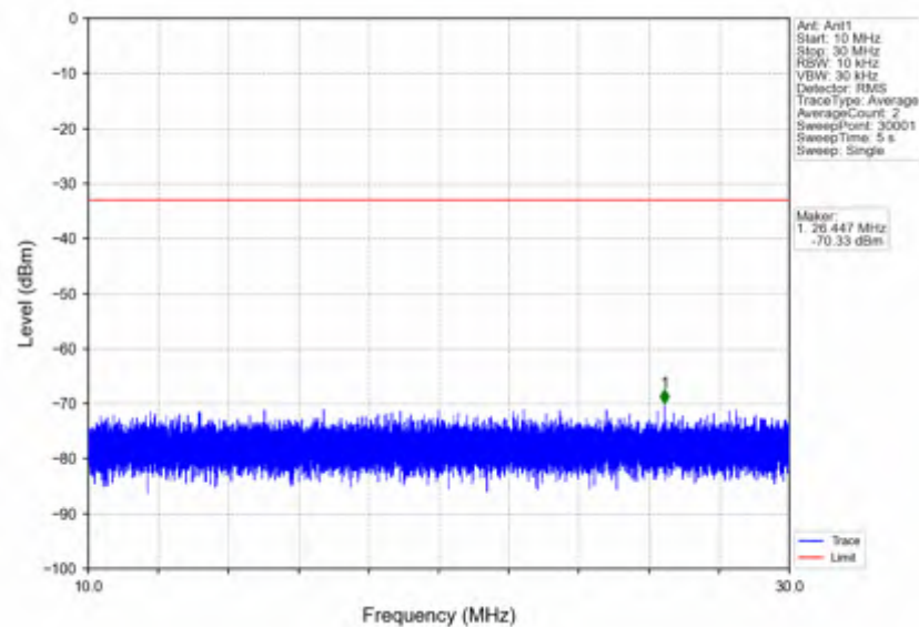
n5_30kHz_SISO_NTNV_15MHz_DFT-s-OFDM PI/2 BPSK_841.5MHz_Outer_Full
