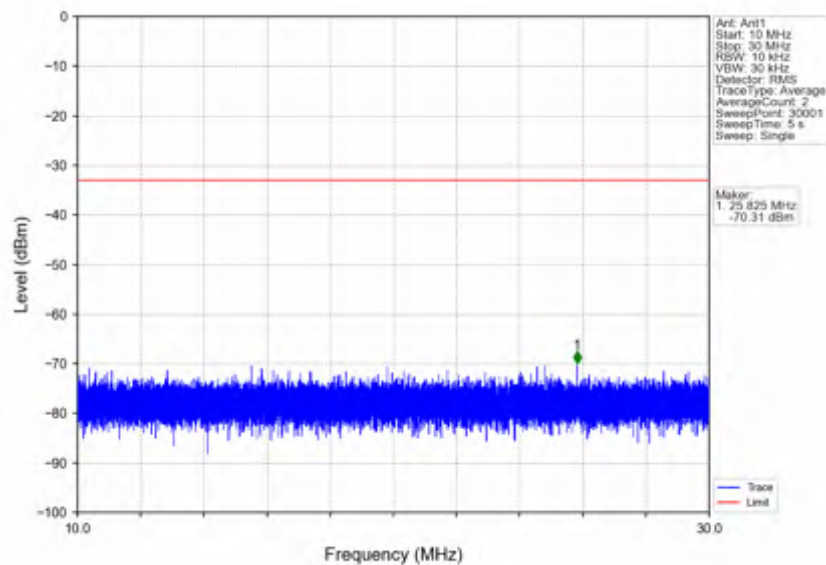
n5_30kHz_SISO_NTNV_10MHz_CP-OFDM QPSK_829MHz_Outer_Full
