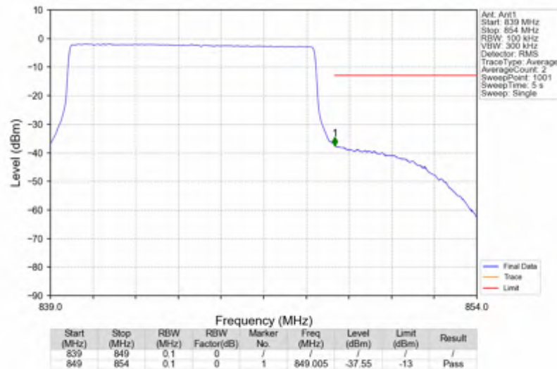
n5_30kHz_SISO_NTNV_10MHz_CP-OFDM QPSK_844MHz_Outer_Full
