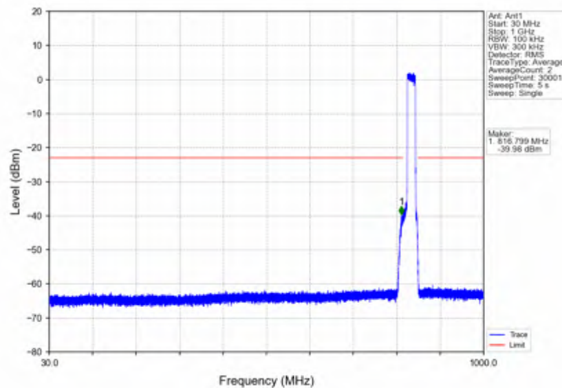
n5_30kHz_SISO_NTNV_20MHz_DFT-s-OFDM QPSK_839MHz_Outer_Full
