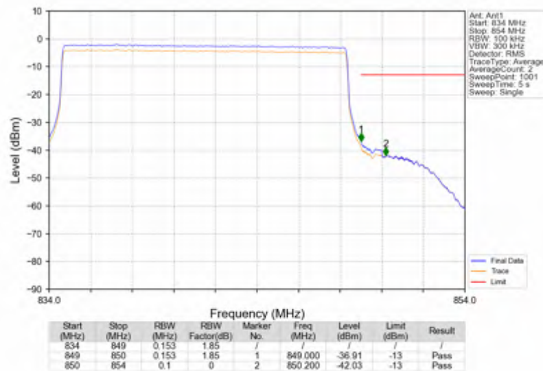
n5_30kHz_SISO_NTV_15MHz_CP-OFDM_QPSK_841.5MHz_Outer_Full
