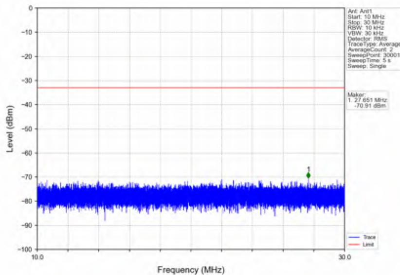
n5_30kHz_SISO_NTNV_15MHz_DFT-s-OFDM_QPSK_831.5MHz_Outer_Full
