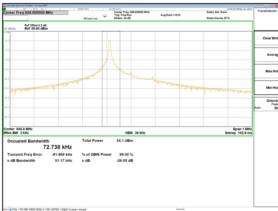
Band26-26dB/99% OBW-27038 Channel-BPSK-1@0-3.75K
