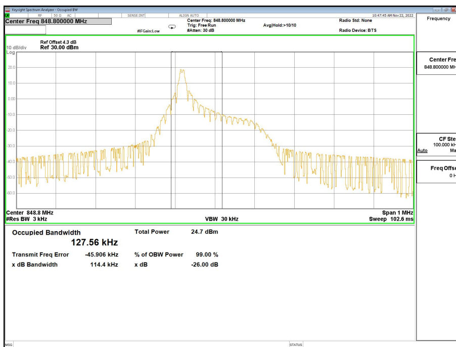
Band26-26dB/99% OBW-27038 Channel-BPSK-1@0-15K
