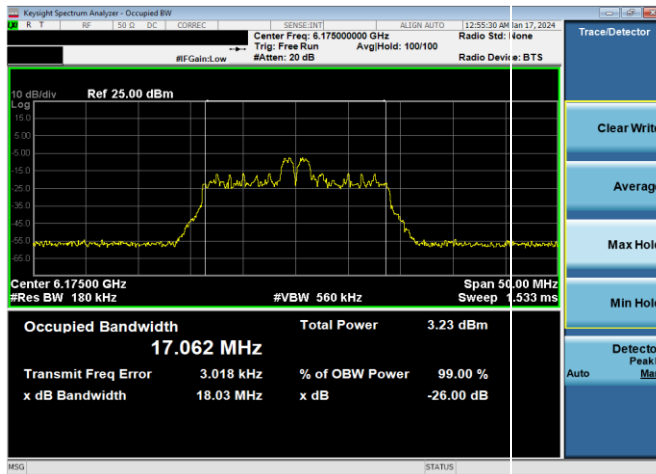
Plot 7-130. 26dB & 99% Bandwidth Plot Antenna WF7 (20MHz 802.11ax RU26 (UNII Band 5) – Ch. 45)
