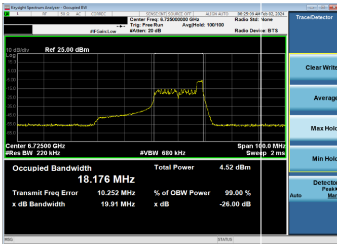
Plot 7-103. 26dB & 99% Bandwidth Plot Antenna WF8 (40MHz 802.11ax RU26 (UNII Band 7) – Ch. 155)
