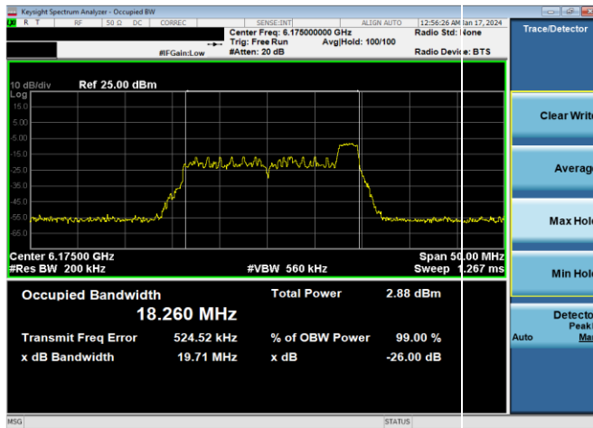
Plot 7-131. 26dB & 99% Bandwidth Plot Antenna WF7 (20MHz 802.11ax RU26 (UNII Band 5) – Ch. 45)
