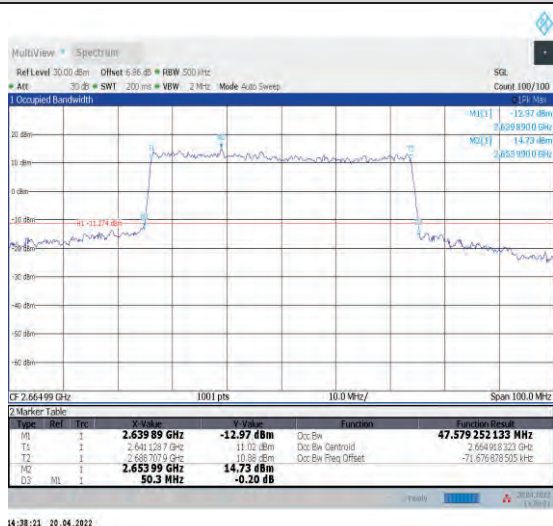
1-N41--30-50-H-8-CP-64QAM-Outer_Full-133@0-Ant t1-47.579-50.300-≤50-PASS
