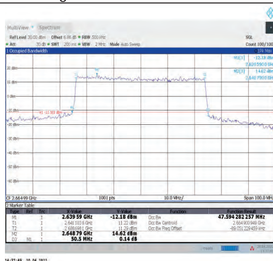
1-N41--30-50-H-7-CP-16QAM-Outer_Full-133@0-An t1-47.594-50.500-≤50-PASS
