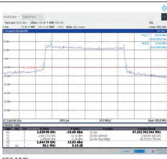
1-N41--30-50-H-6-CP-QPSK-Outer_Full-133@0-Ant t1-47.533-50.100-≤50-PASS
