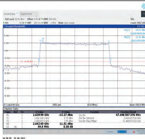
1-N41--30-50-H-9-CP-256QAM-Outer_Full-133@0-A nt1-47.499-49.900-≤50-PASS
