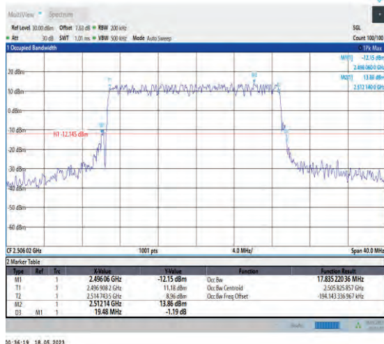
1-N41-PC1-30-20-L-1-DFT-QPSK-Outer_Full-50@ Ant1-17.835-19.480-≤20-PASS
