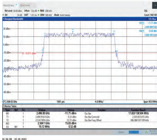
1-N41-PC1-30-20-L-3-DFT-16QAM-Outer_Full-50@ 0-Ant1-17.833-19.120-≤20-PASS
