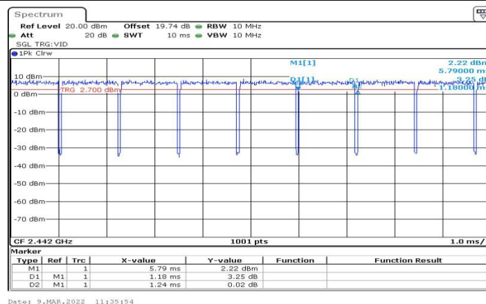
11N20SISO_Ant1_2442
