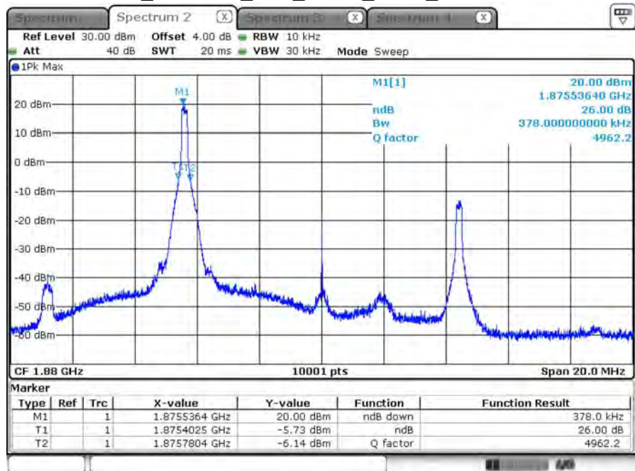
B2_CH18900_10M_QPSK_1RB0_26dB BW
