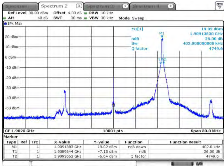
B2_CH19125_15M_16-QAM_1RB74_26dB BW
