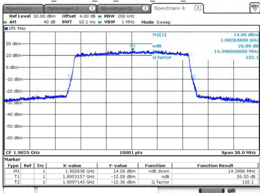
B2_CH19125_15M_16-QAM_75RB0_26dB BW
