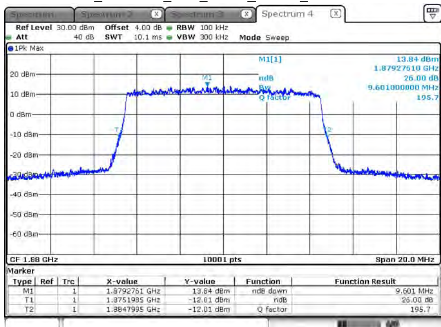
B2_CH18900_10M_QPSK_50RB0_26dB BW
