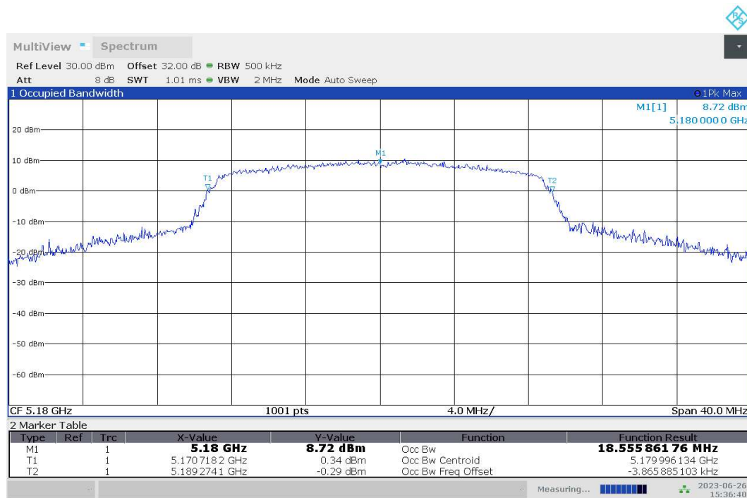
Fig.21 99% Occupied bandwidth (802.11n-HT20, 5180MHz)
