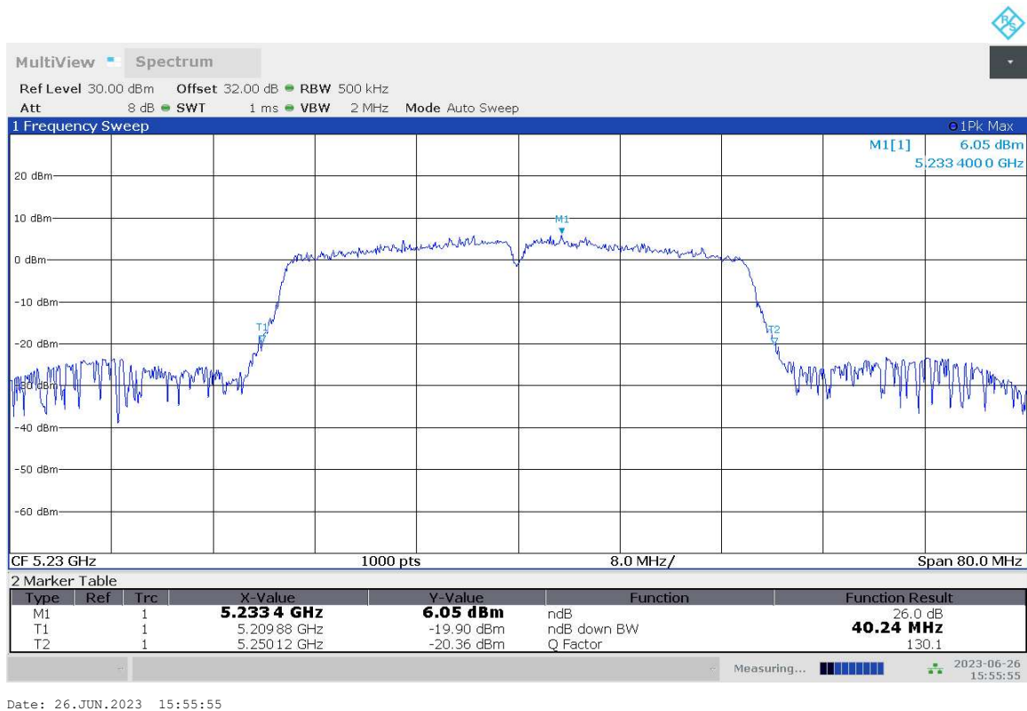
Fig.8 Occupied 26dB Bandwidth (802.11n-HT40, 5230MHz)
