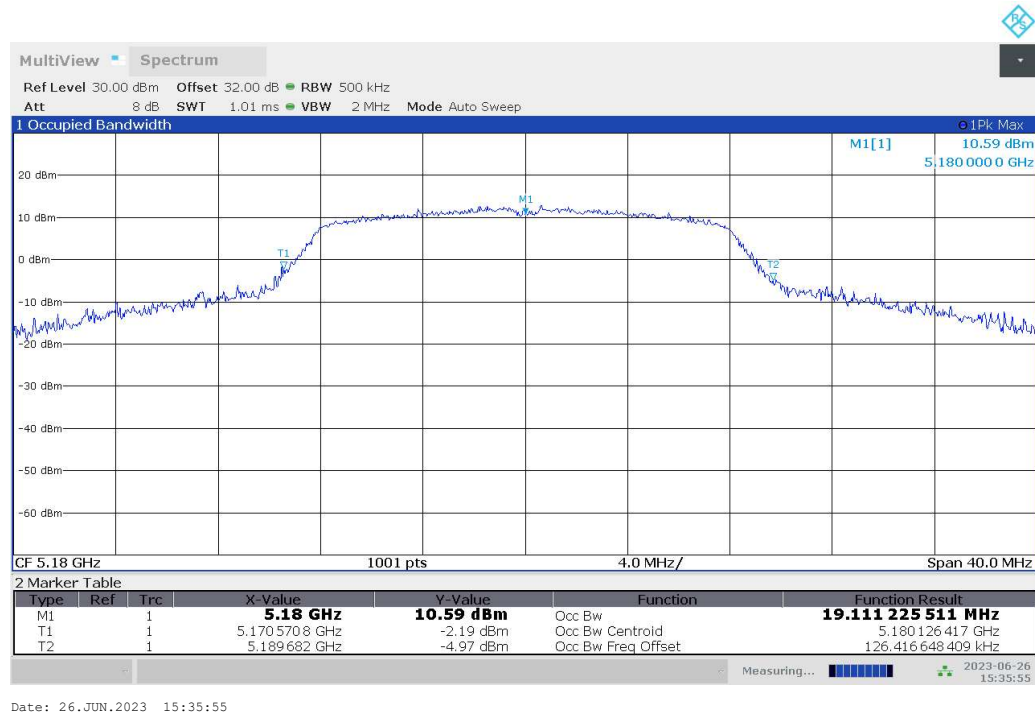
Fig.18 99% Occupied bandwidth (802.11a, 5180MHz)
