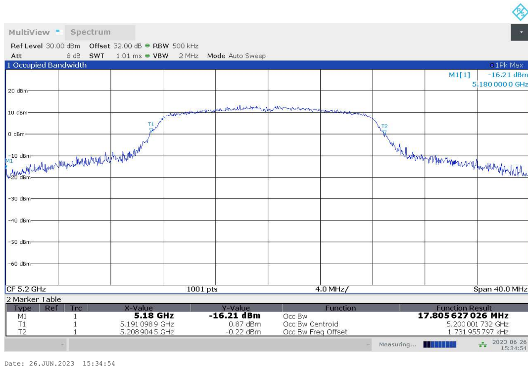
Fig.19 99% Occupied bandwidth (802.11a, 5200MHz)
