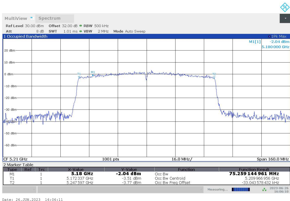
Fig.26 99% Occupied bandwidth (802.11ac-HT80, 5210MHz)
