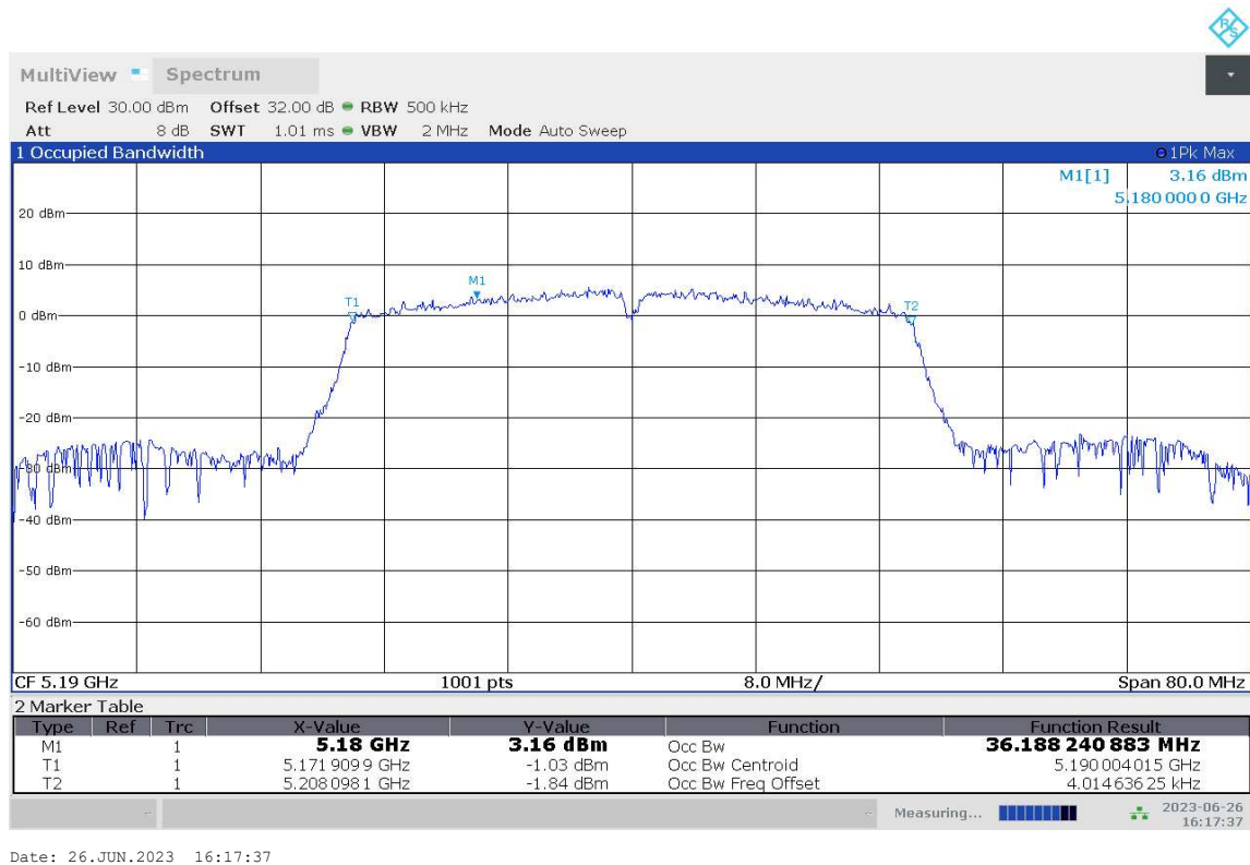
Fig.24 99% Occupied bandwidth (802.11n-HT40, 5190MHz)
