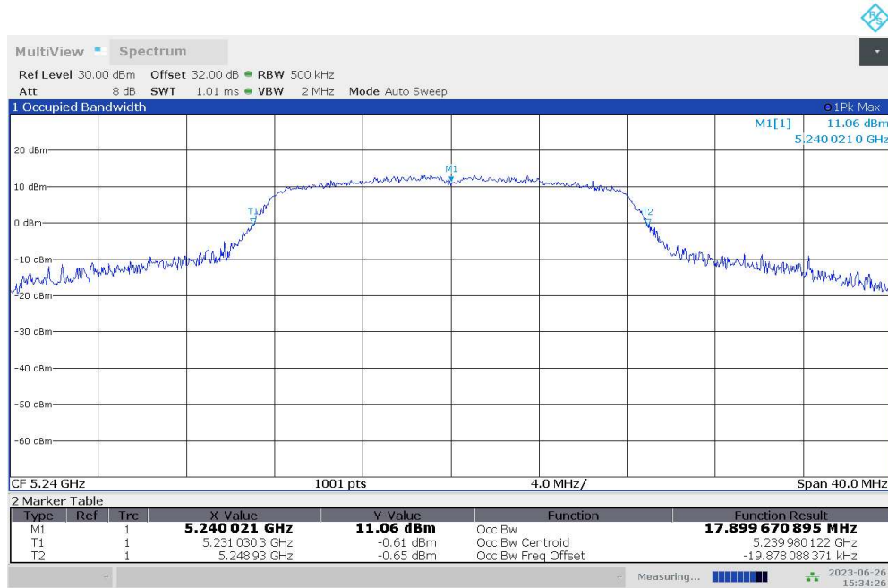
Fig.20 99% Occupied bandwidth (802.11a, 5240MHz)
