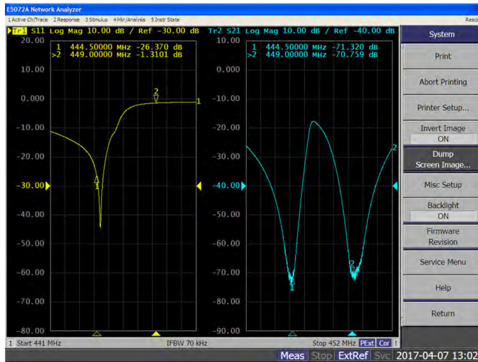
Figure 27: Rejection of Each Port for UHF Duplexer
