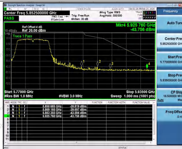
11AC40MIMO_Ant2_High_5795
