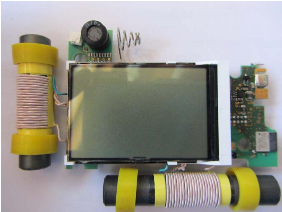
Figure 3: PIEPS MICRO, Front side
