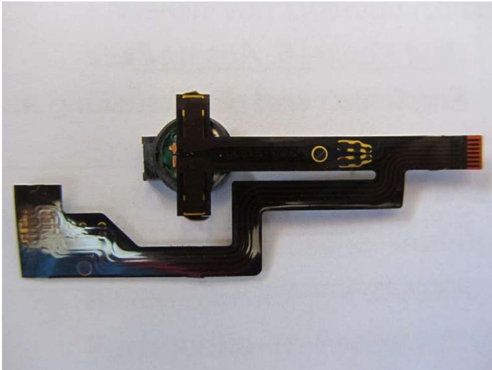
Figure 7: PIEPS MICRO - ProxBoard
