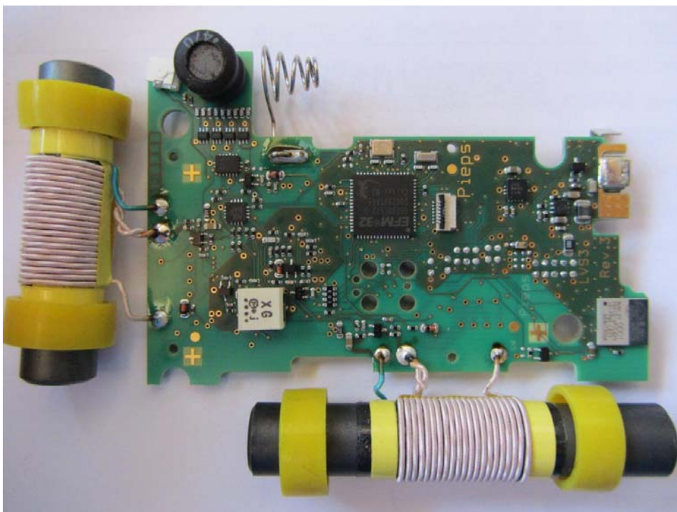
Figure 4: PIEPS MICRO, Front side
