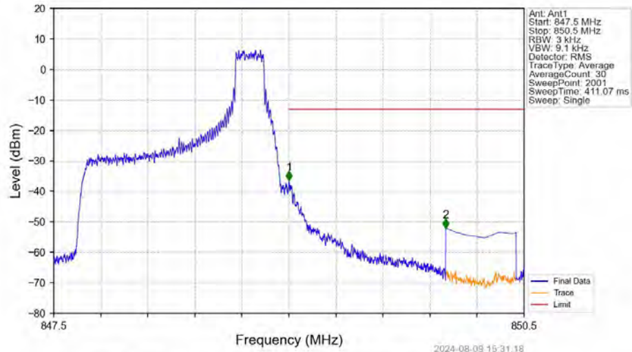
Band5_1.4MHz_QPSK_HCH_848.3MHz_RB_1_5_NTNV
