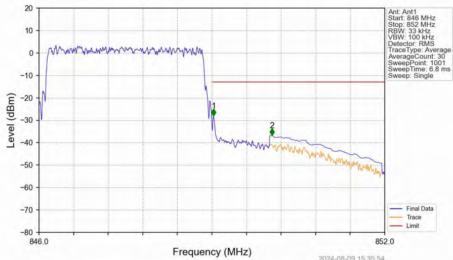
Band5_3MHz_16QAM_HCH_847.5MHz_RB_15_0_NTNV
