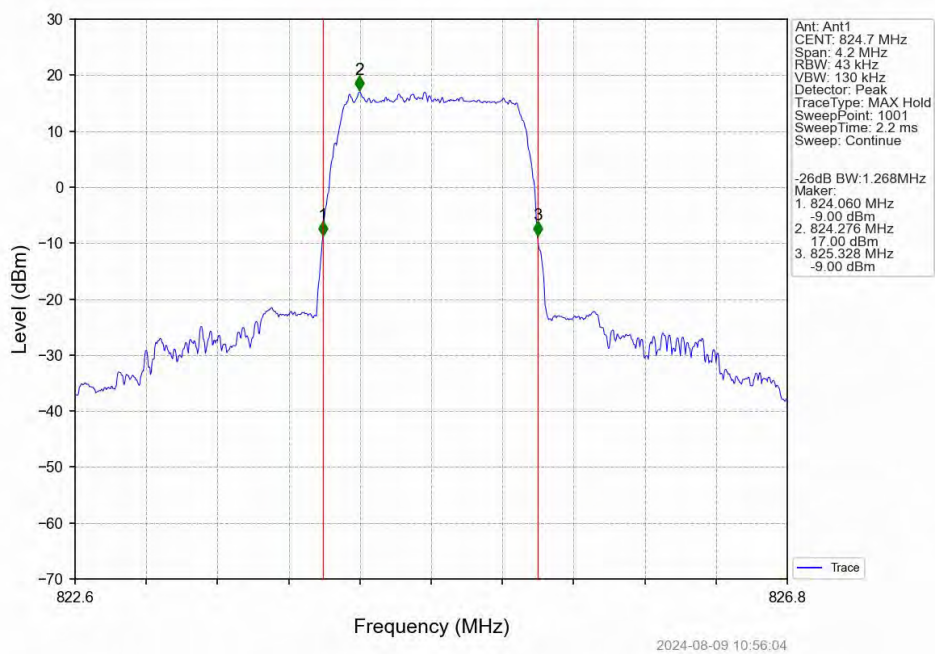
Band5_1.4MHz_16QAM_LCH_824.7MHz_RB_6_0_NTNV
