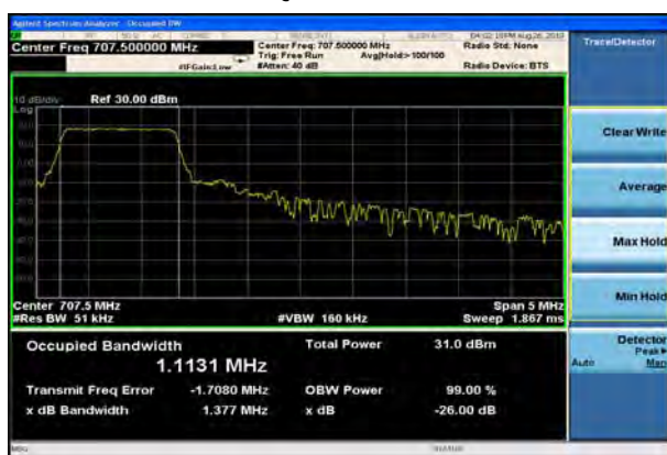
LTE Band 12 16QAM 1.4MHz CH-Middle
