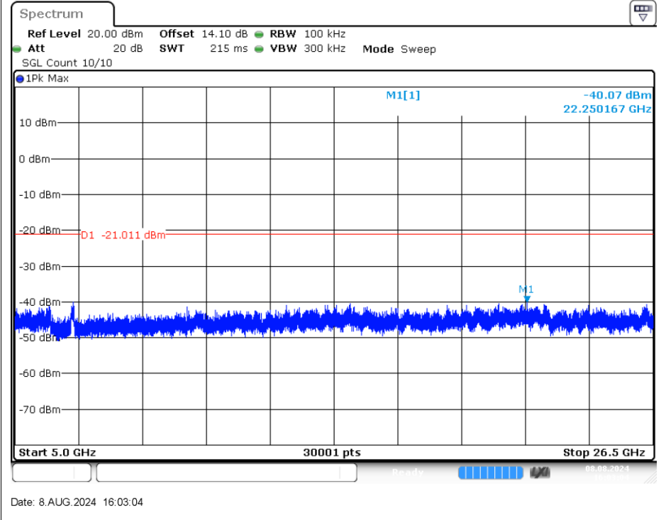
Tx. Spurious NVNT 3-DH5 2402MHz Ant1 Emission Range3
