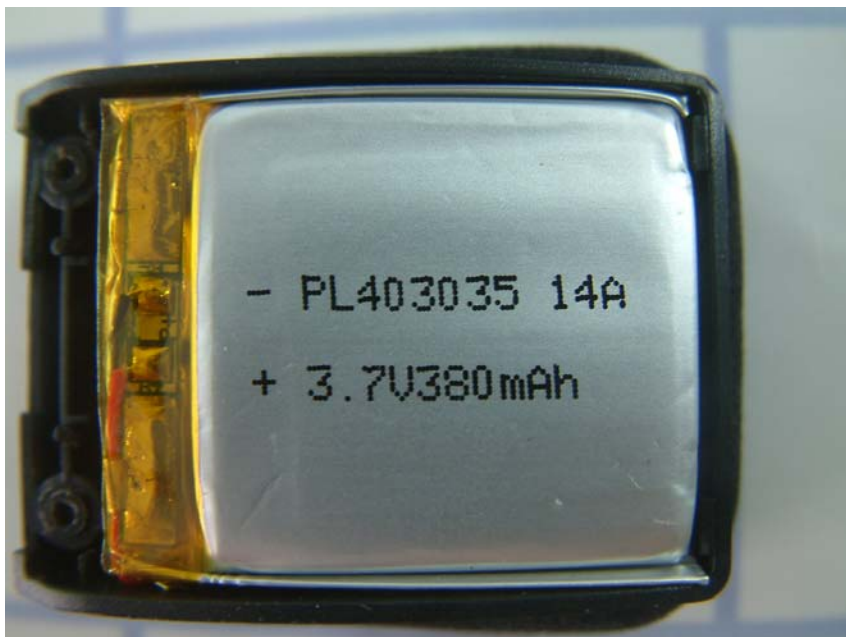
Battery view
