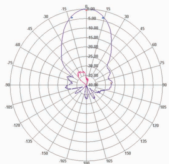
Azimuth (E-plane) Co- and Cross- Polarization Radiation Patterns
