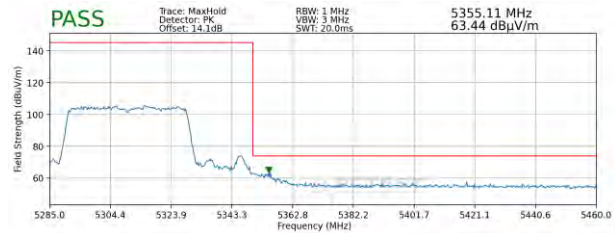
Plot 7-304. Radiated Upper Band Edge Plot MIMO (Peak - UNII Band 2A) - WCP
