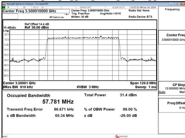
Band77-Part27_60MHz_DFT_s_OFDM_SCS30kHz_BPSK_RB162_0_CH633334
