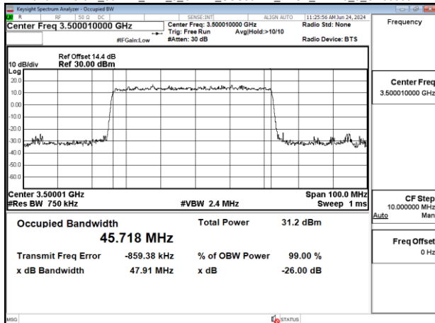
Band77-Part27_50MHz_DFT_s_OFDM_SCS30kHz_BPSK_RB128_0_CH633334
