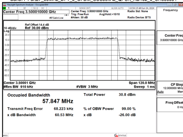
Band77-Part27_60MHz_DFT_s_OFDM_SCS30kHz_QPSK_RB162_0_CH633334
