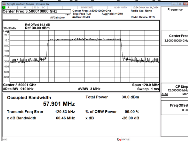
Band77-Part27_60MHz_DFT_s_OFDM_SCS30kHz_16QAM_RB162_0_CH633334
