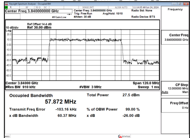
Band77-Part27_60MHz_DFT_s_OFDM_SCS30kHz_BPSK_RB162_0_CH656000
