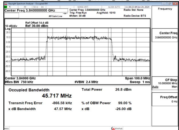
Band77-Part27_50MHz_DFT_s_OFDM_SCS30kHz_BPSK_RB128_0_CH656000
