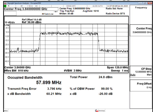
Band77-Part27_60MHz_DFT_s_OFDM_SCS30kHz_16QAM_RB162_0_CH656000
