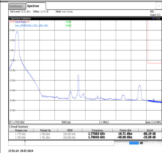
Band66-10MHz-16QAM-132622-1RB#49-PASS
