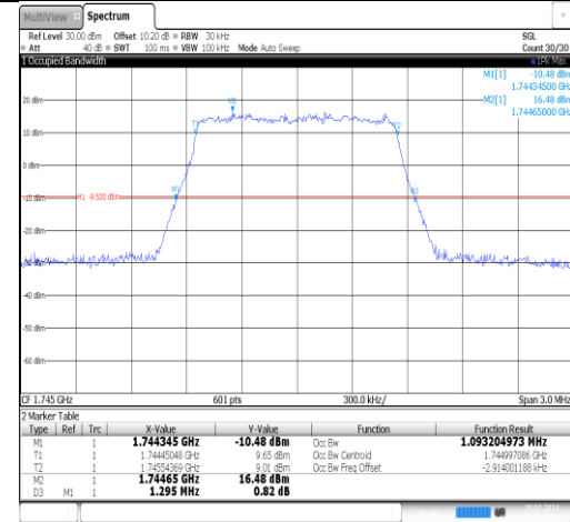
Band66-3MHz-QPSK-132322-15RB#0-PASS
