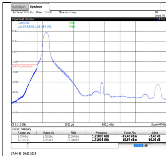
Band66-5MHz-16QAM-131997-1RB#24-PASS
