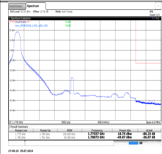
Band66-5MHz-16QAM-132647-1RB#24-PASS
