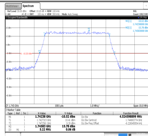
Band66-5MHz-QPSK-132322-25RB#0-PASS
