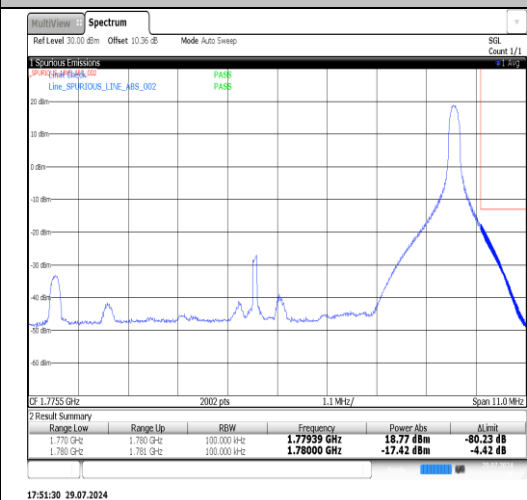
Band66-15MHz-QPSK-132047-75RB#0-PASS
