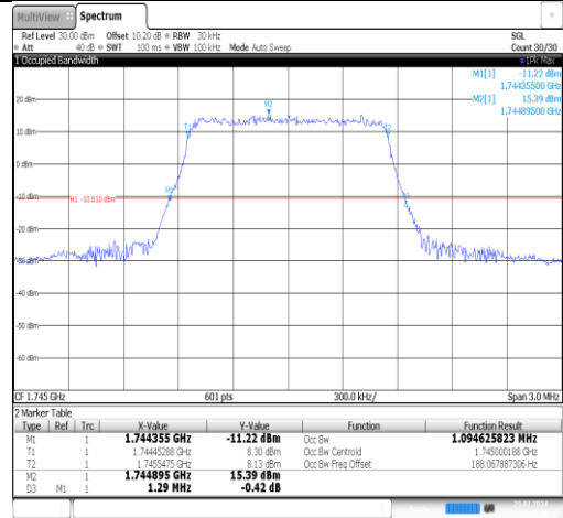
Band66-1.4MHz-16QAM-132322-6RB#0-PASS
