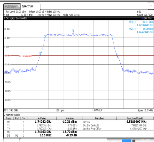
Band66-5MHz-16QAM-132322-25RB#0-PASS
