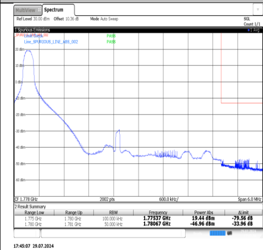
Band66-5MHz-QPSK-132647-1RB#24-PASS
