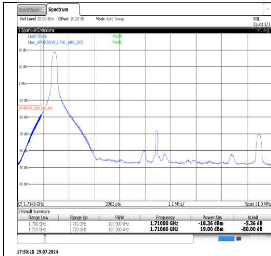
Band66-10MHz-16QAM-132022-1RB#49-PASS
