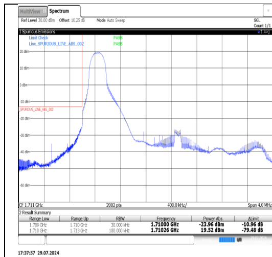
Band66-3MHz-16QAM-131987-1RB#14-PASS
