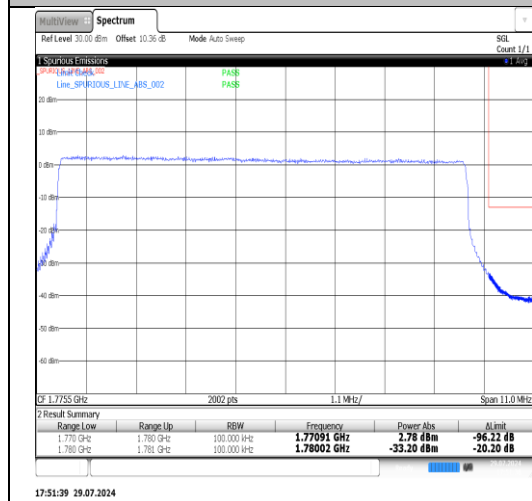
Band66-10MHz-QPSK-132622-50RB#0-PASS
