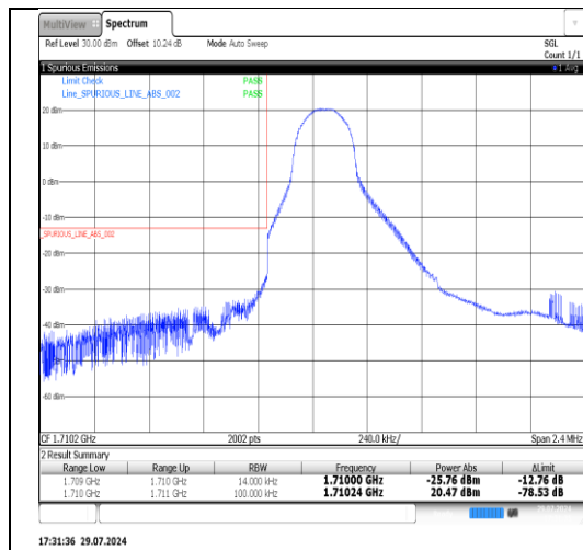
Band66-1.4MHz-QPSK-131979-1RB#5-PASS
