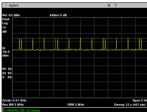
Plot 17. DFS Calibration, Radar Type 5, 5510 MHz
