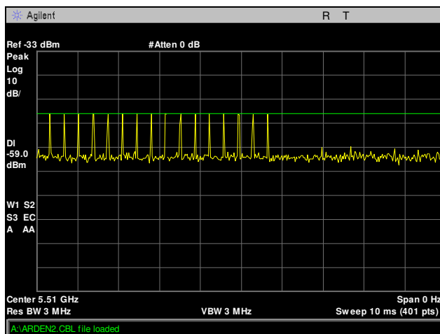
Plot 15. DFS Calibration, Radar Type 3, 5510 MHz
