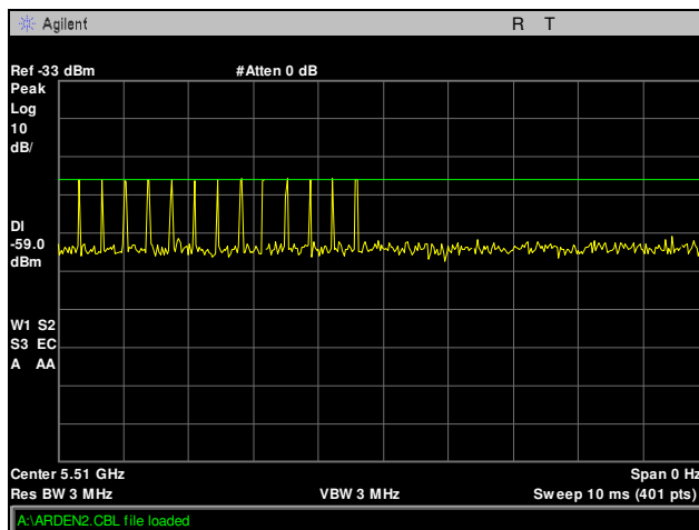
Plot 16. DFS Calibration, Radar Type 4, 5510 MHz
