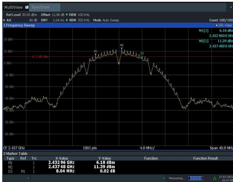
Fig.A.4.2 Occupied 6dB Bandwidth (802.11b, Ch 6)
