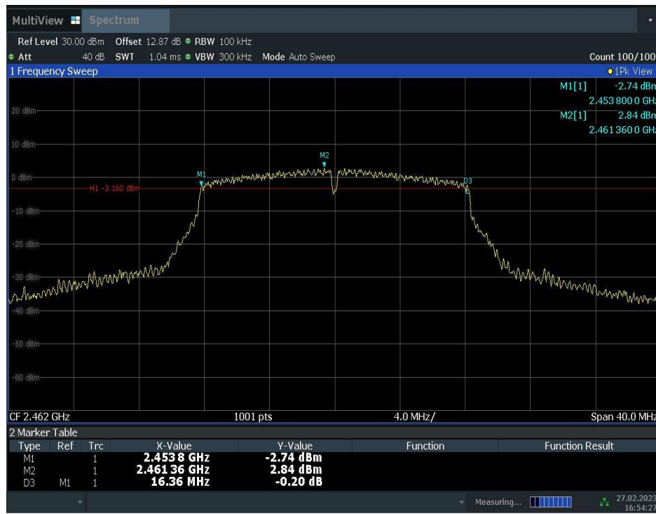
Fig.A.4.6 Occupied 6dB Bandwidth (802.11g, Ch 11)
