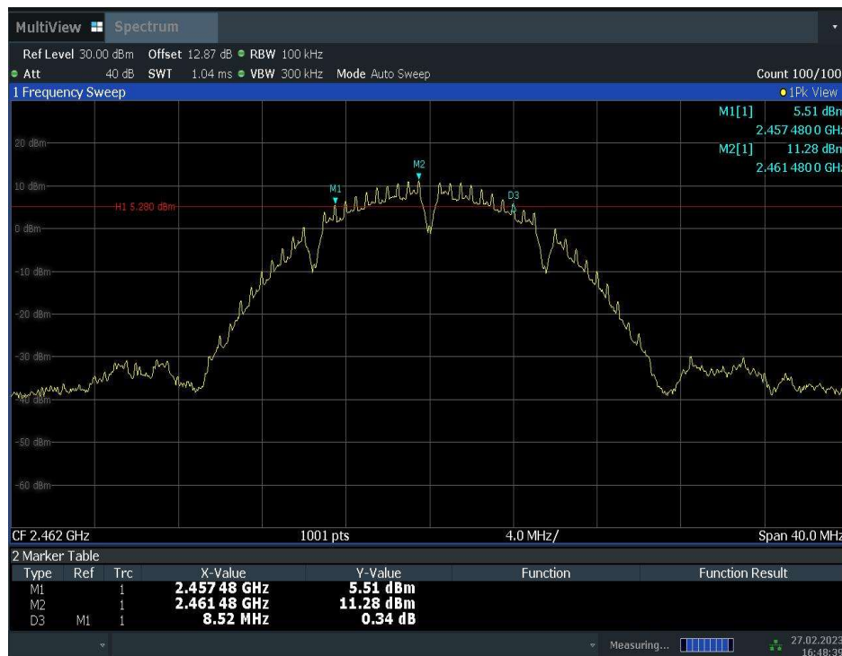
Fig.A.4.3 Occupied 6dB Bandwidth (802.11b, Ch 11)
