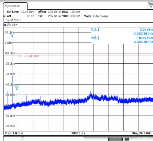
BLE_2M-Ant1-2402-0~Reference-PASS
