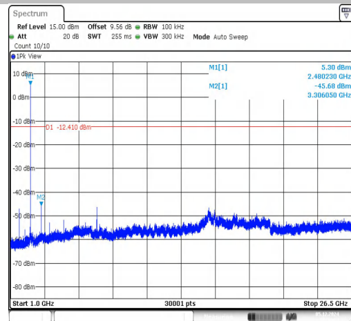
BLE_2M-Ant1-2480-0~Reference-PASS
