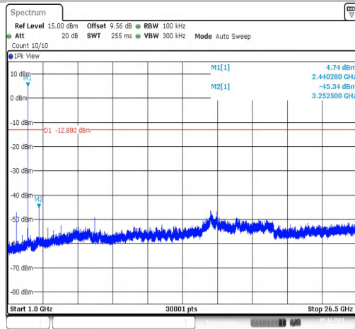
BLE_2M-Ant1-2440-0~Reference-PASS
