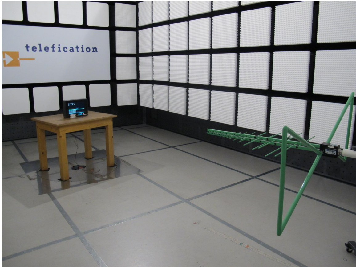
Photograph 3: Test setup radiated emissions (0.03 - 1 GHz)
