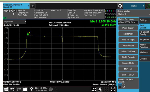
Channel 207 (6985MHz)
