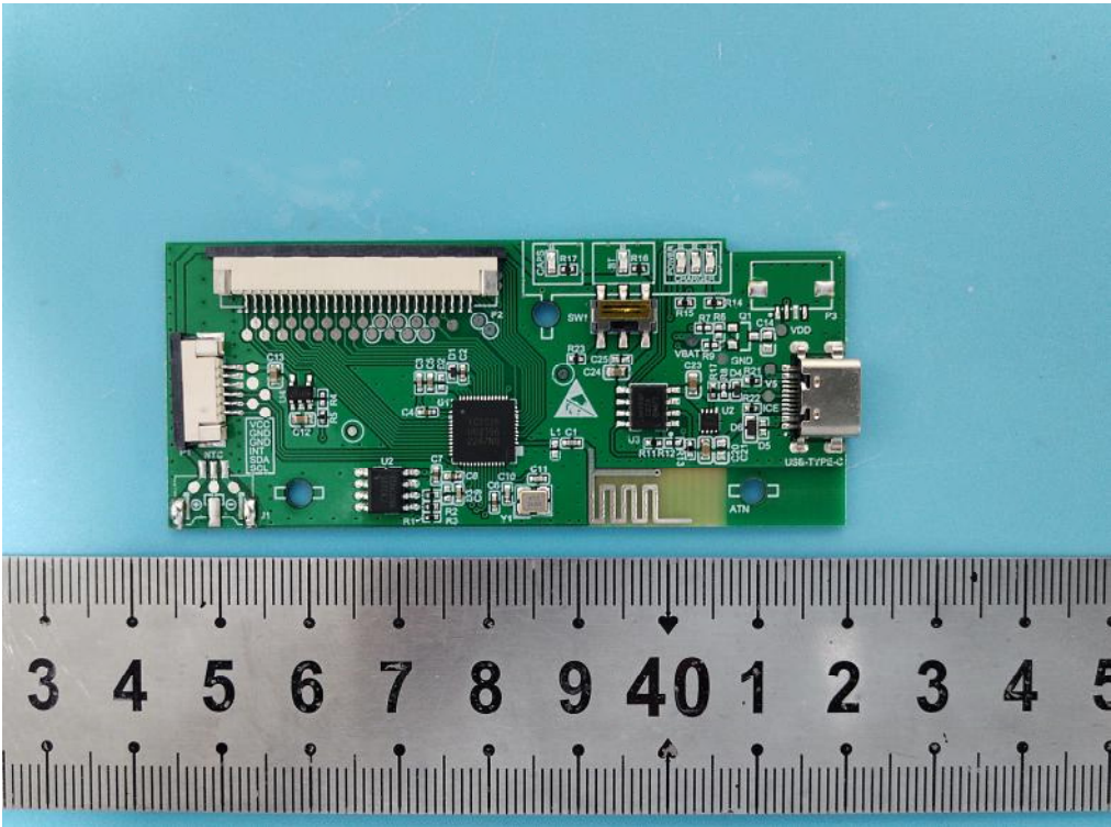
BT&BLE Chip
