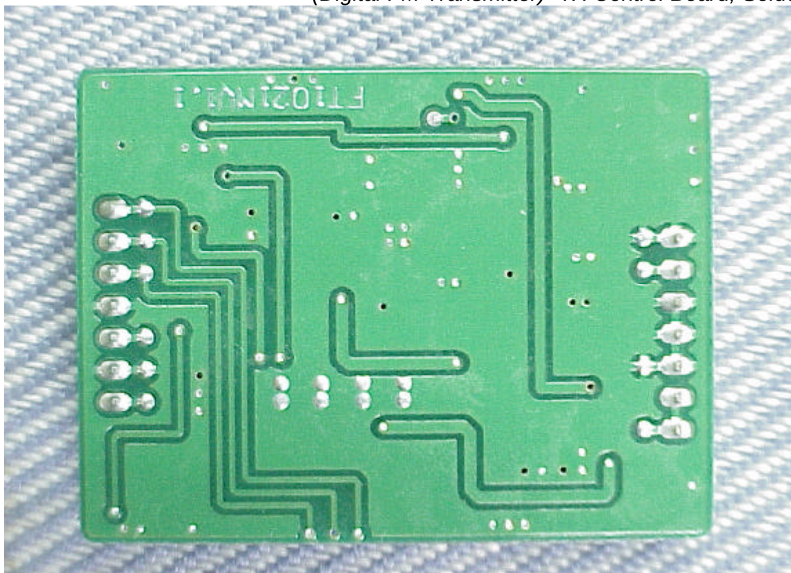
Photo 17 (Digital FM Transmitter) TX Control Board, Solder Side
