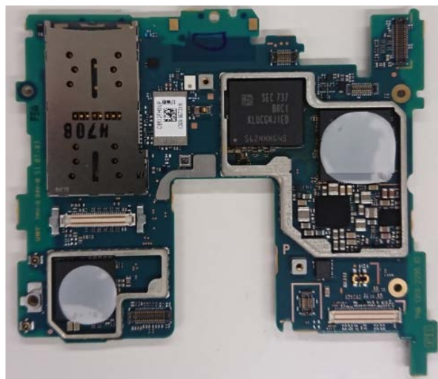
Internal PWB without Shield cases (Front-side)
