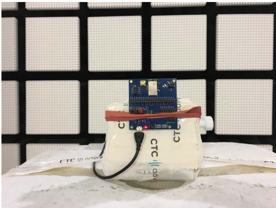
Photo 4: radiated emission above 1GHz
