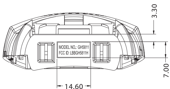
GH5811 HANDSET
