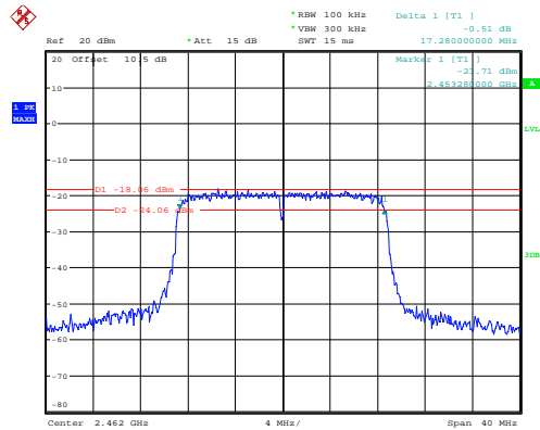
802.11n ht20_2462MHz
