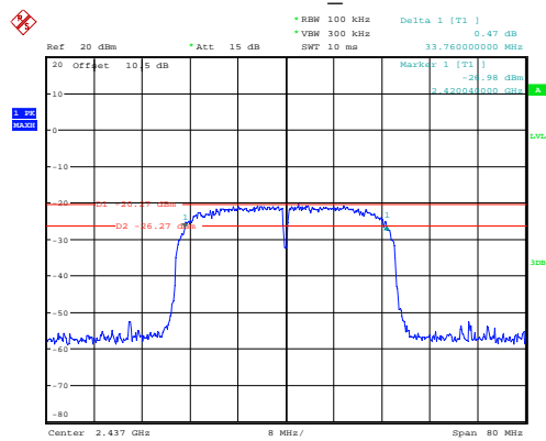
802.11n ht40_2437MHz
