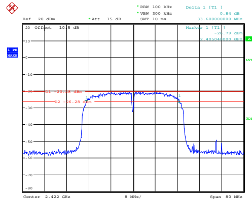
802.11n ht40_2422MHz
