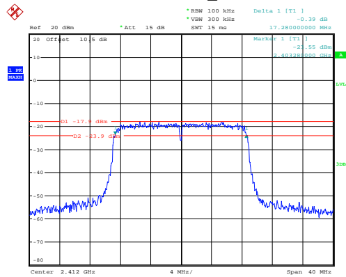
802.11n ht20_2412MHz
