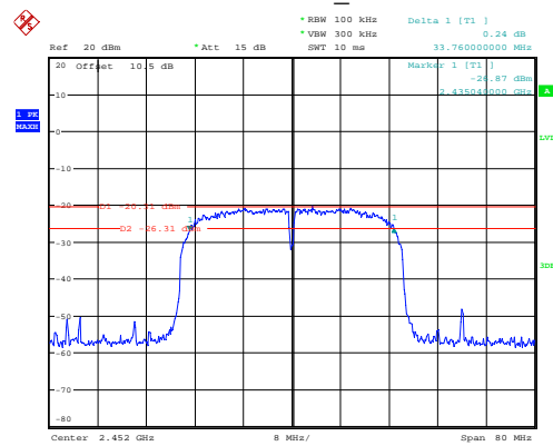
802.11n ht40_2452MHz
