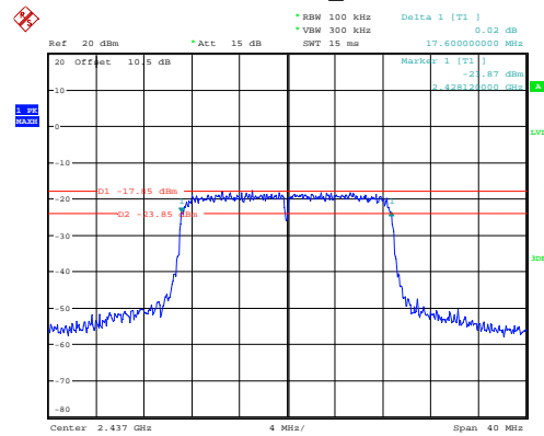
802.11n ht20_2437MHz
