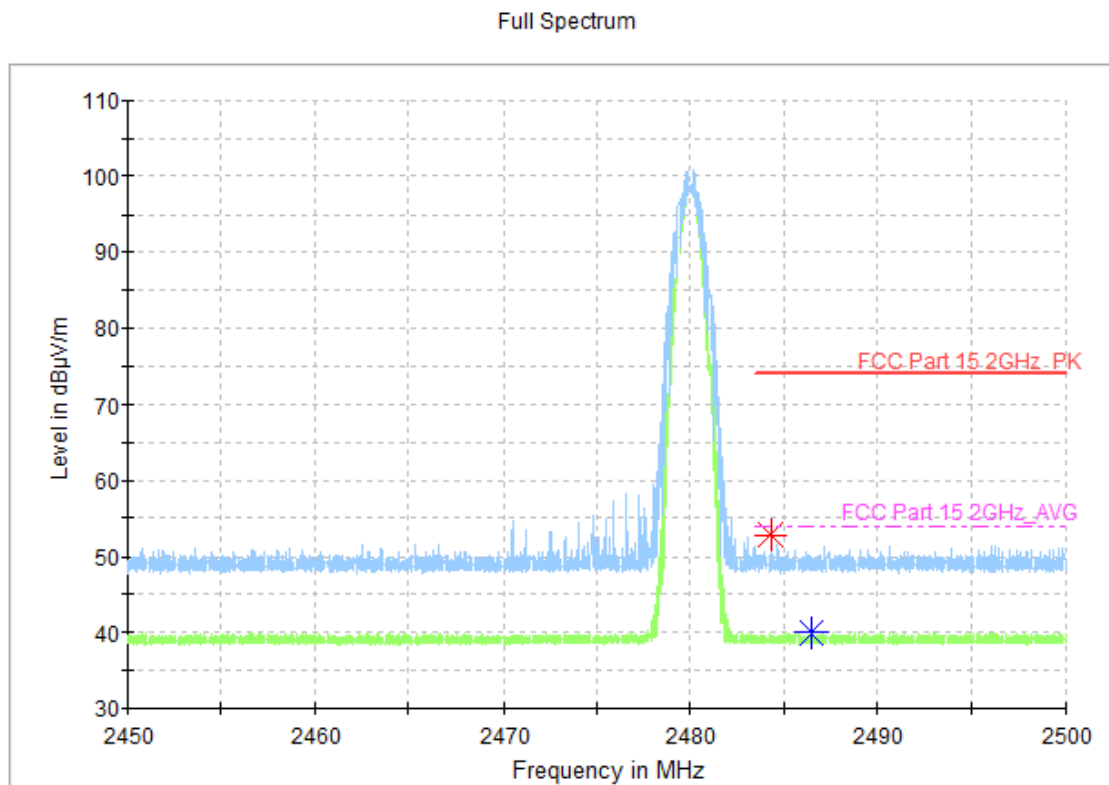
Fig.63. Frequency Band Edges: 8DPSK, Channel 78, 2.45 GHz - 2.50GHz
